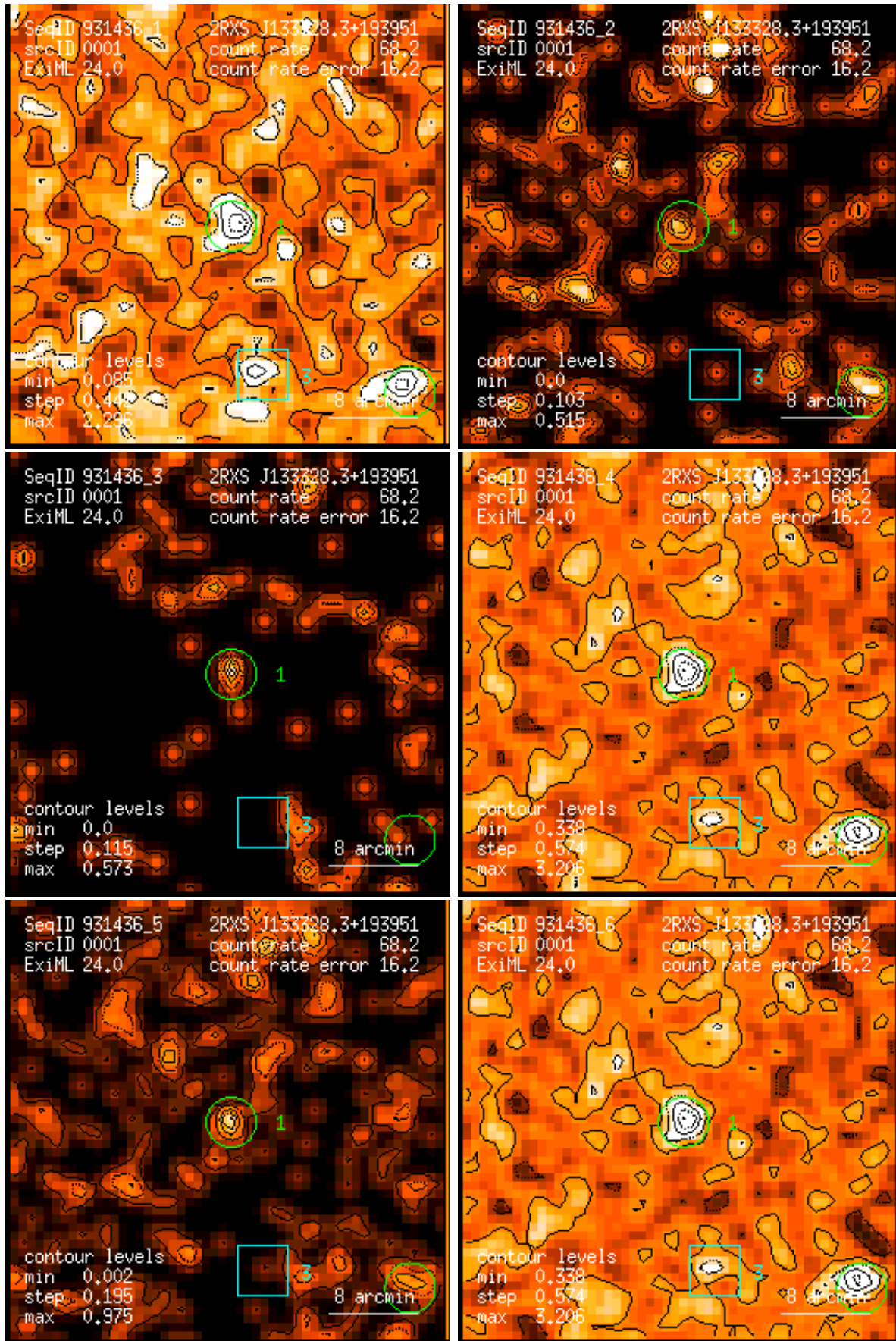
Figure 1: RASS 931436: detection 0001: band rate images, Gaussian filter: (1) PSPC channels 11 – 41, (2) 52 – 90, (3) 91 – 201, (4) 11 – 235, (5) 52 – 201, (6) 11 – 201. Broad band rates in counts/ks. Band rate contour levels in counts/ks/arcmin 2 .
