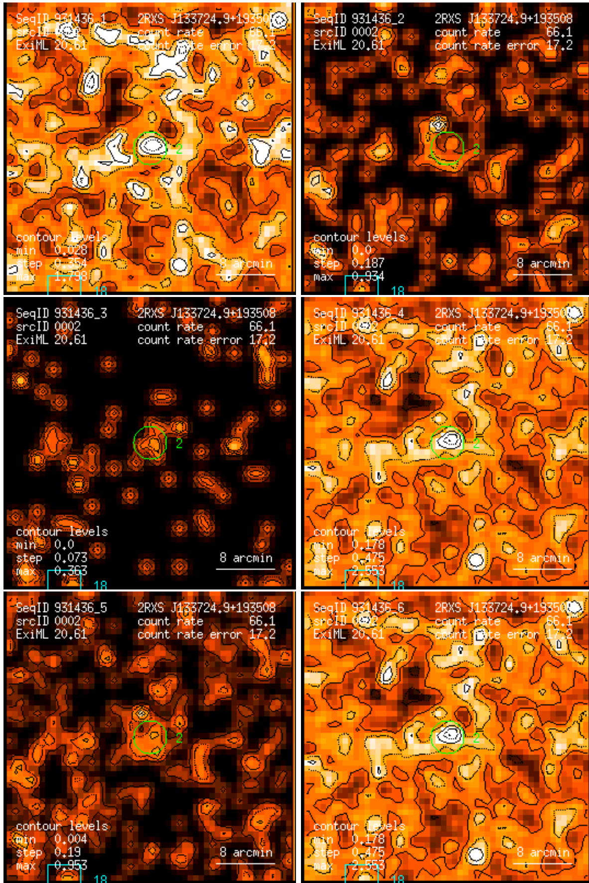
Figure 2: RASS 931436: detection 0002: band rate images, Gaussian filter: (1) PSPC channels 11 – 41, (2) 52 – 90, (3) 91 – 201, (4) 11 – 235, (5) 52 – 201, (6) 11 – 201. Broad band rates in counts/ks. Band rate contour levels in counts/ks/arcmin 2 .
