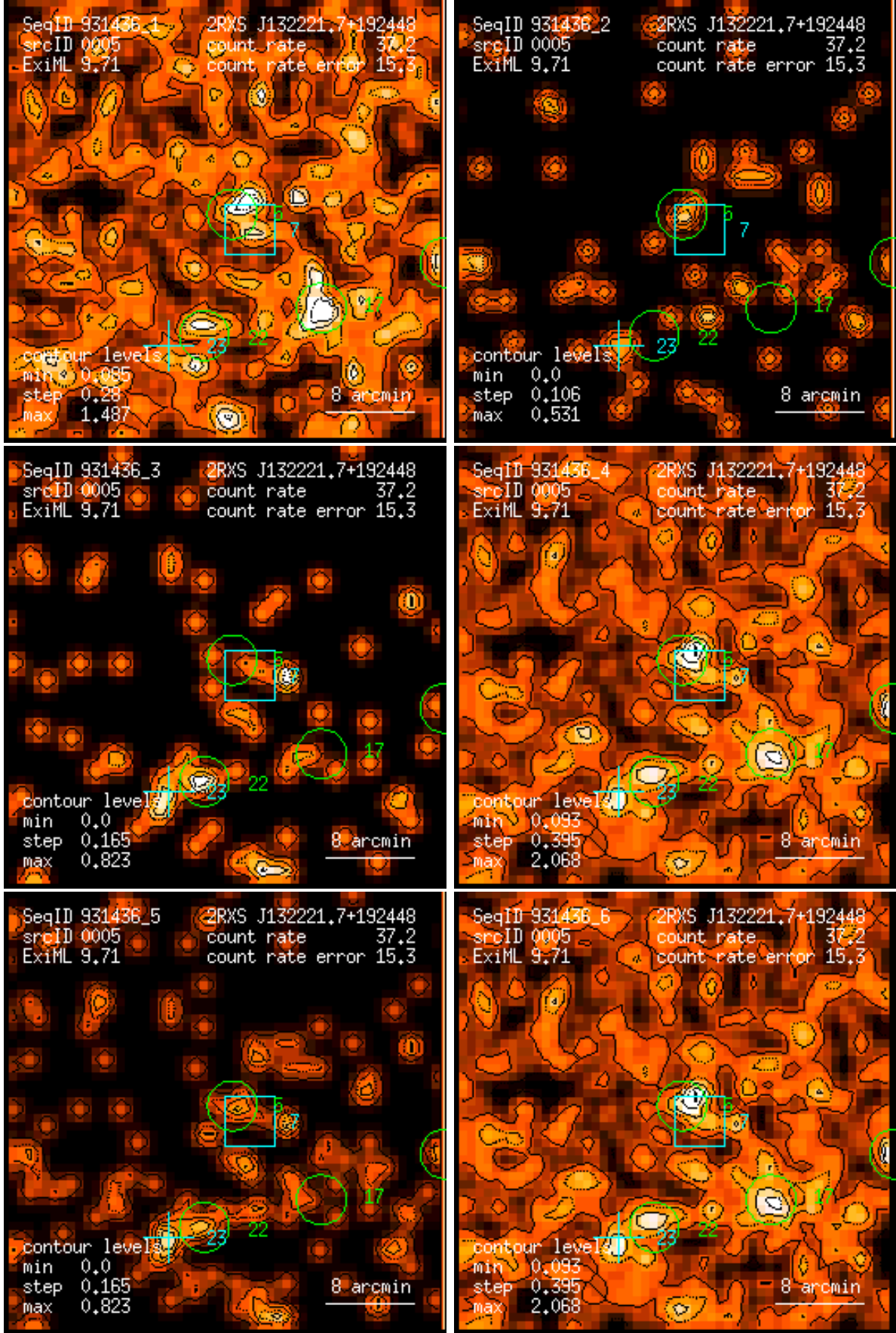
Figure 5: RASS 931436: detection 0005: band rate images, Gaussian filter: (1) PSPC channels 11 – 41, (2) 52 – 90, (3) 91 – 201, (4) 11 – 235, (5) 52 – 201, (6) 11 – 201. Broad band rates in counts/ks. Band rate contour levels in counts/ks/arcmin 2 .
