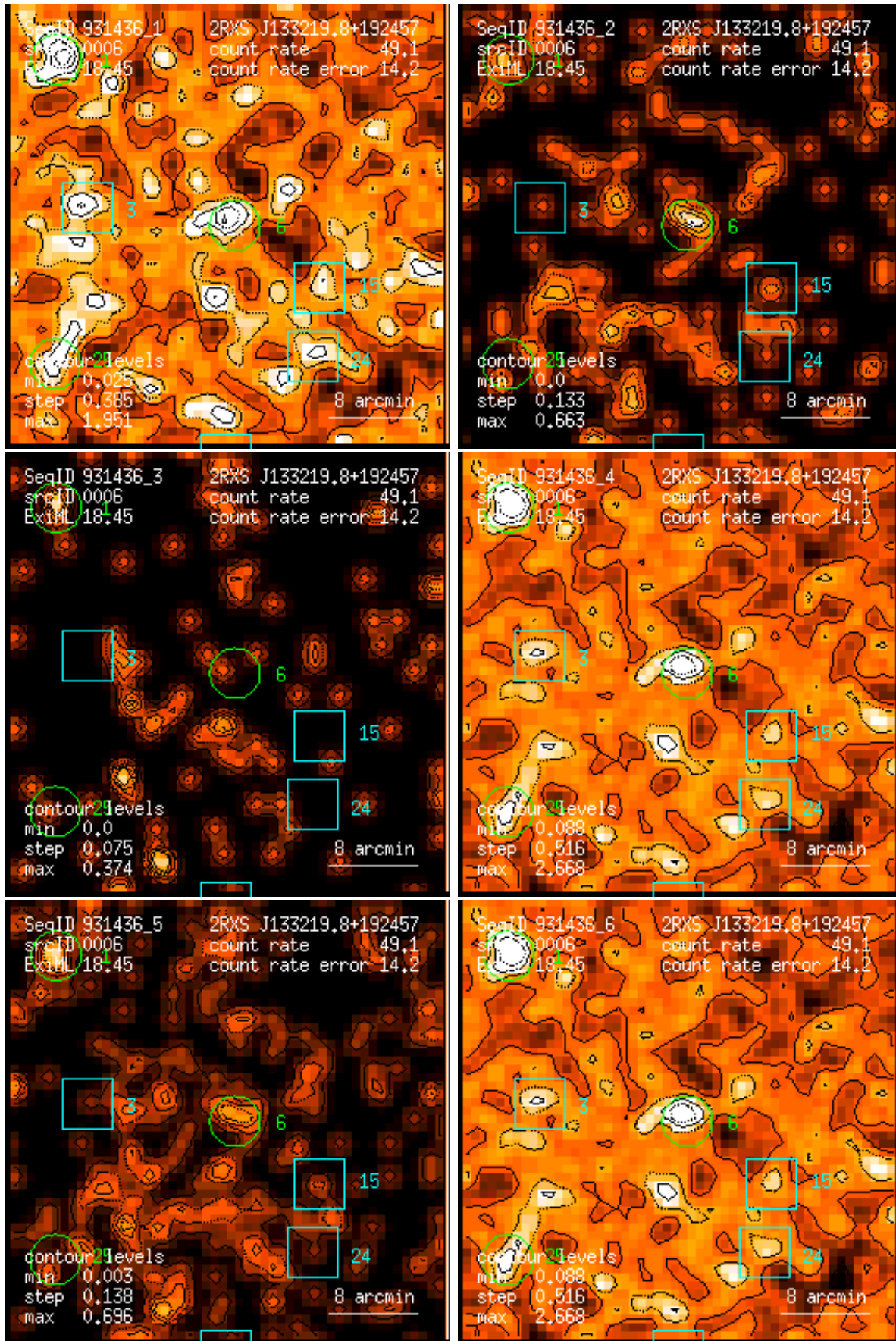
Figure 6: RASS 931436: detection 0006: band rate images, Gaussian filter: (1) PSPC channels 11 – 41, (2) 52 – 90, (3) 91 – 201, (4) 11 – 235, (5) 52 – 201, (6) 11 – 201. Broad band rates in counts/ks. Band rate contour levels in counts/ks/arcmin 2 .
