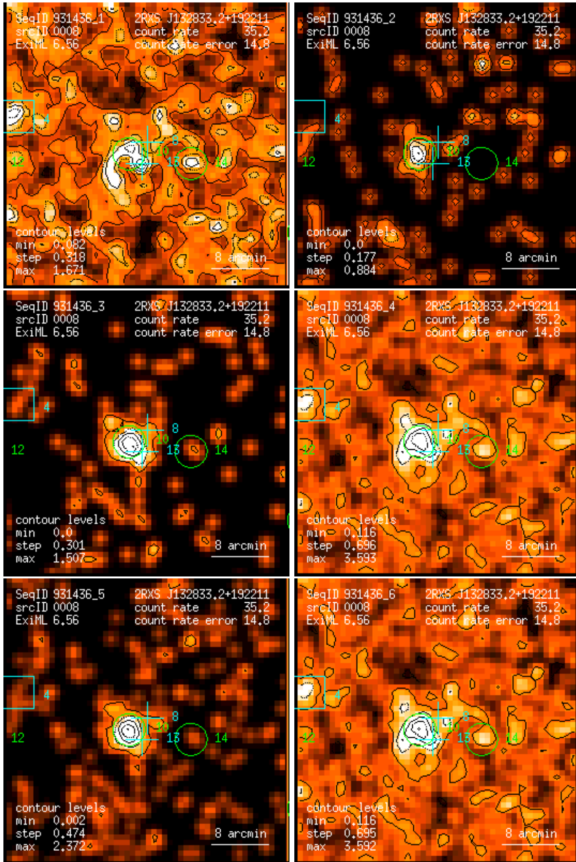
Figure 8: RASS 931436: detection 0008: band rate images, Gaussian filter: (1) PSPC channels 11 – 41, (2) 52 – 90, (3) 91 – 201, (4) 11 – 235, (5) 52 – 201, (6) 11 – 201. Broad band rates in counts/ks. Band rate contour levels in counts/ks/arcmin 2 .
