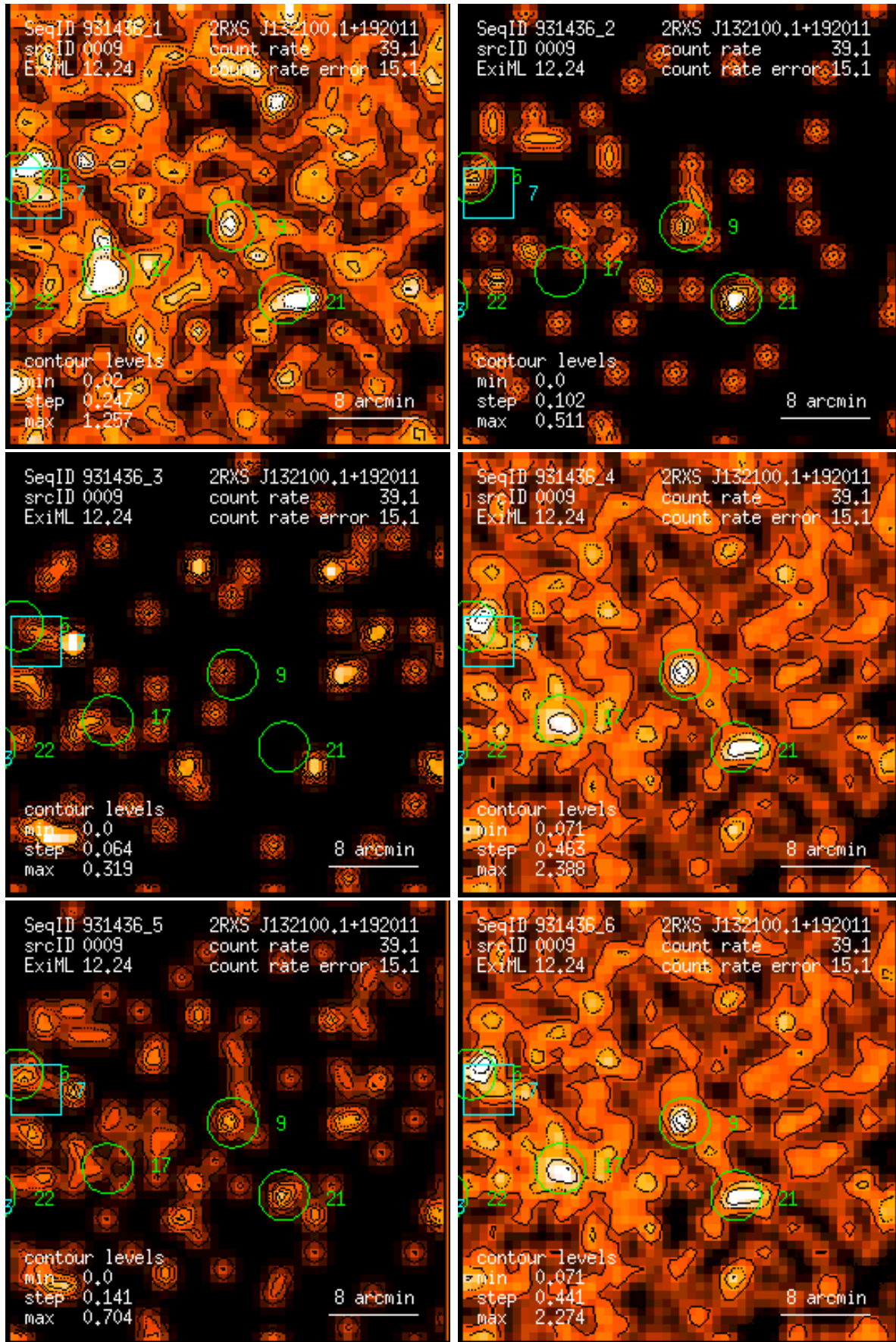
Figure 9: RASS 931436: detection 0009: band rate images, Gaussian filter: (1) PSPC channels 11 – 41, (2) 52 – 90, (3) 91 – 201, (4) 11 – 235, (5) 52 – 201, (6) 11 – 201. Broad band rates in counts/ks. Band rate contour levels in counts/ks/arcmin 2 .
