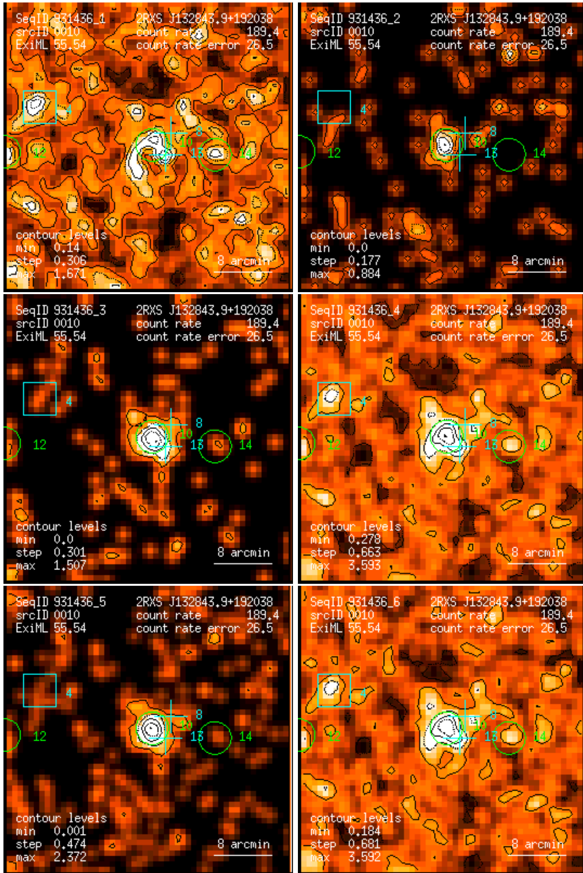
Figure 10: RASS 931436: detection 0010: band rate images, Gaussian filter: (1) PSPC channels 11 – 41, (2) 52 – 90, (3) 91 – 201, (4) 11 – 235, (5) 52 – 201, (6) 11 – 201. Broad band rates in counts/ks. Band rate contour levels in counts/ks/arcmin 2 .
