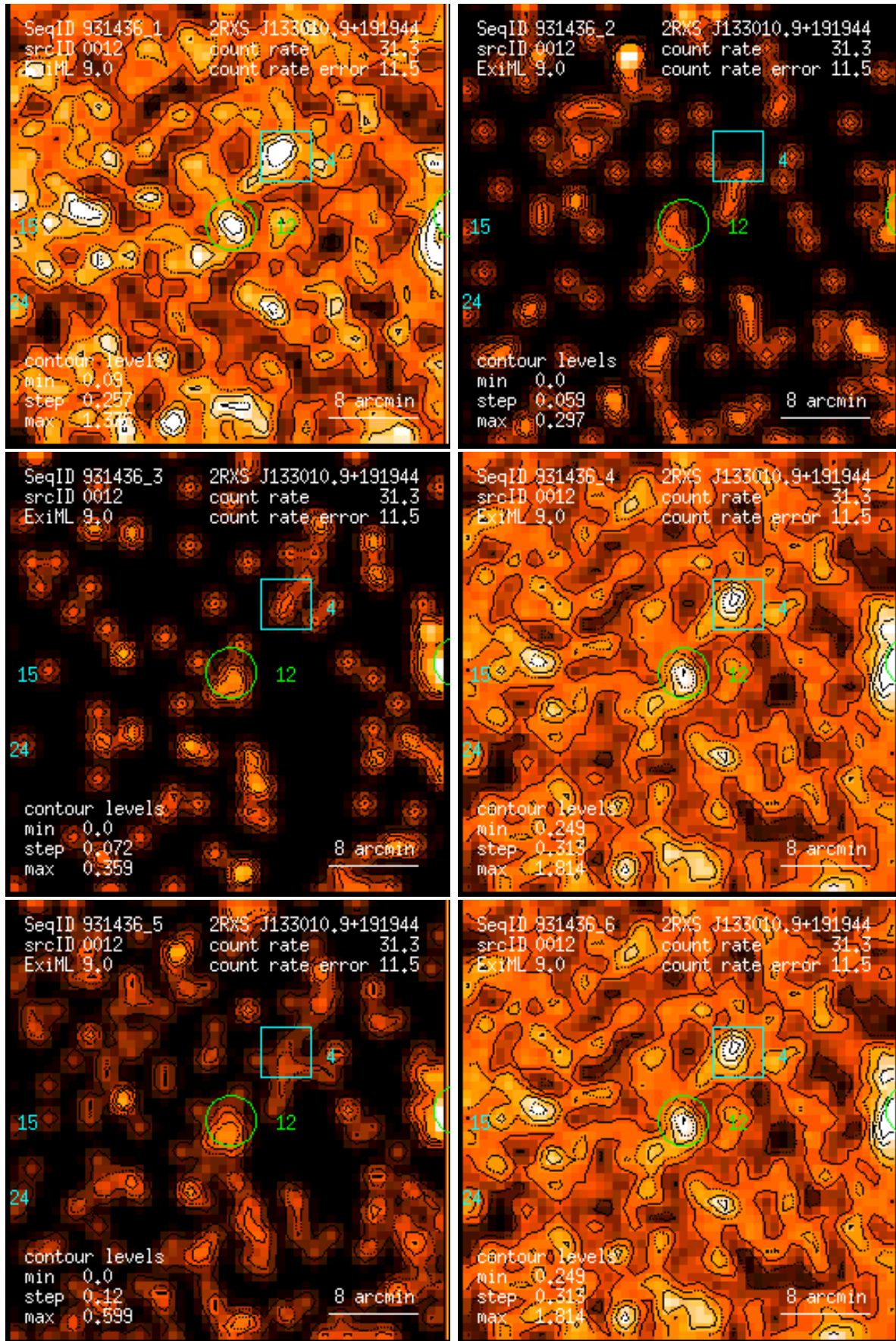
Figure 12: RASS 931436: detection 0012: band rate images, Gaussian filter: (1) PSPC channels 11 – 41, (2) 52 – 90, (3) 91 – 201, (4) 11 – 235, (5) 52 – 201, (6) 11 – 201. Broad band rates in counts/ks. Band rate contour levels in counts/ks/arcmin 2 .
