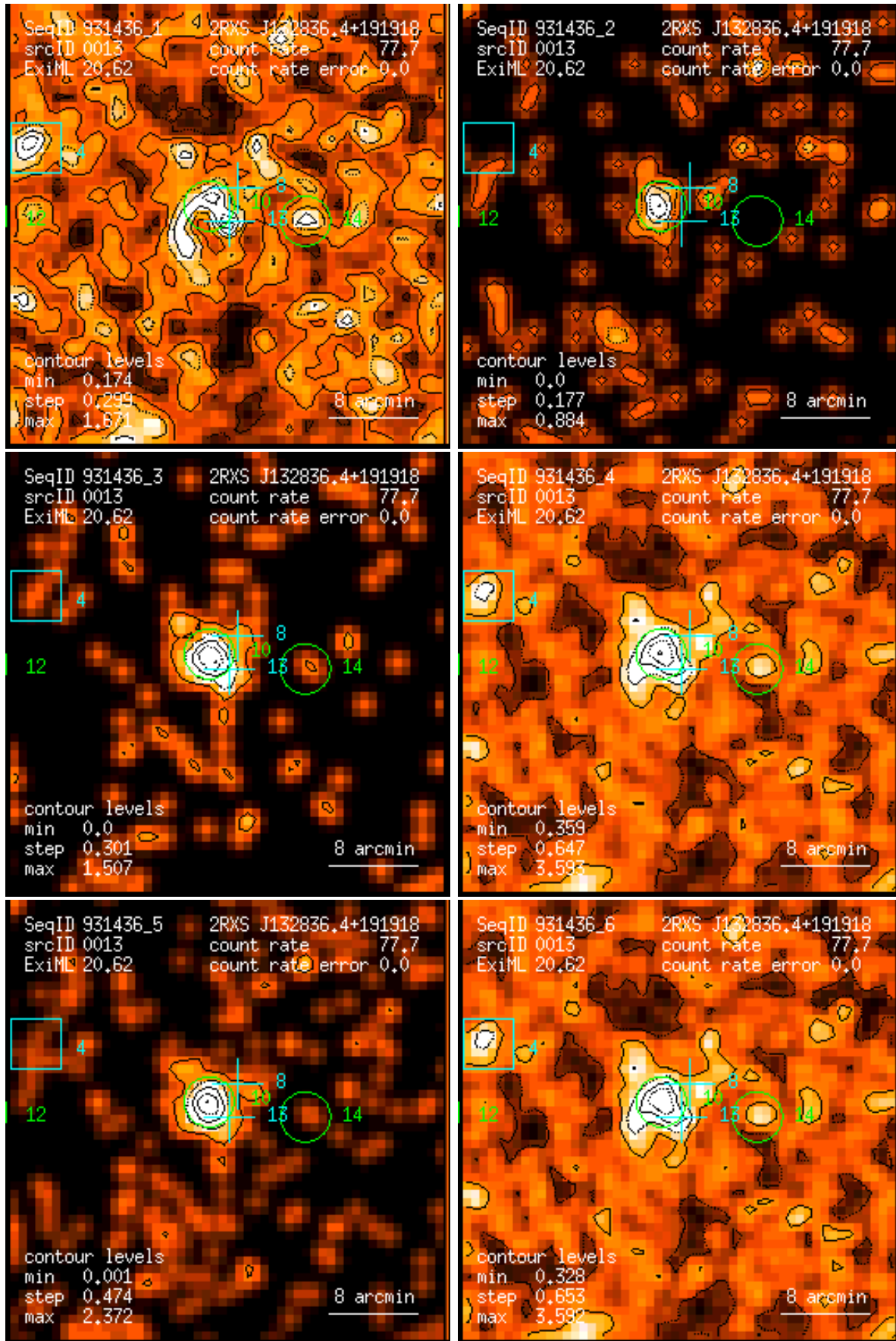
Figure 13: RASS 931436: detection 0013: band rate images, Gaussian filter: (1) PSPC channels 11 – 41, (2) 52 – 90, (3) 91 – 201, (4) 11 – 235, (5) 52 – 201, (6) 11 – 201. Broad band rates in counts/ks. Band rate contour levels in counts/ks/arcmin 2 .
