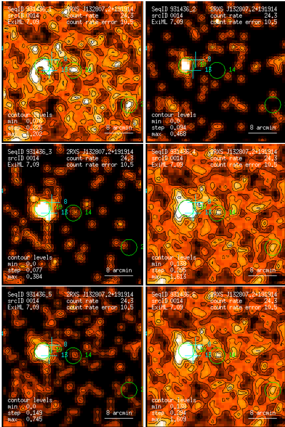
Figure 14: RASS 931436: detection 0014: band rate images, Gaussian filter: (1) PSPC channels 11 – 41, (2) 52 – 90, (3) 91 – 201, (4) 11 – 235, (5) 52 – 201, (6) 11 – 201. Broad band rates in counts/ks. Band rate contour levels in counts/ks/arcmin 2 .
