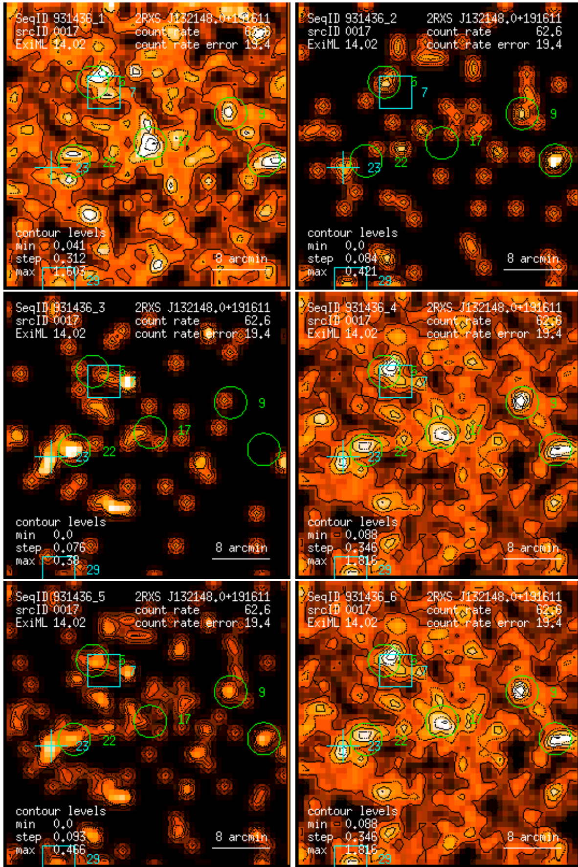
Figure 17: RASS 931436: detection 0017: band rate images, Gaussian filter: (1) PSPC channels 11 – 41, (2) 52 – 90, (3) 91 – 201, (4) 11 – 235, (5) 52 – 201, (6) 11 – 201. Broad band rates in counts/ks. Band rate contour levels in counts/ks/arcmin 2 .
