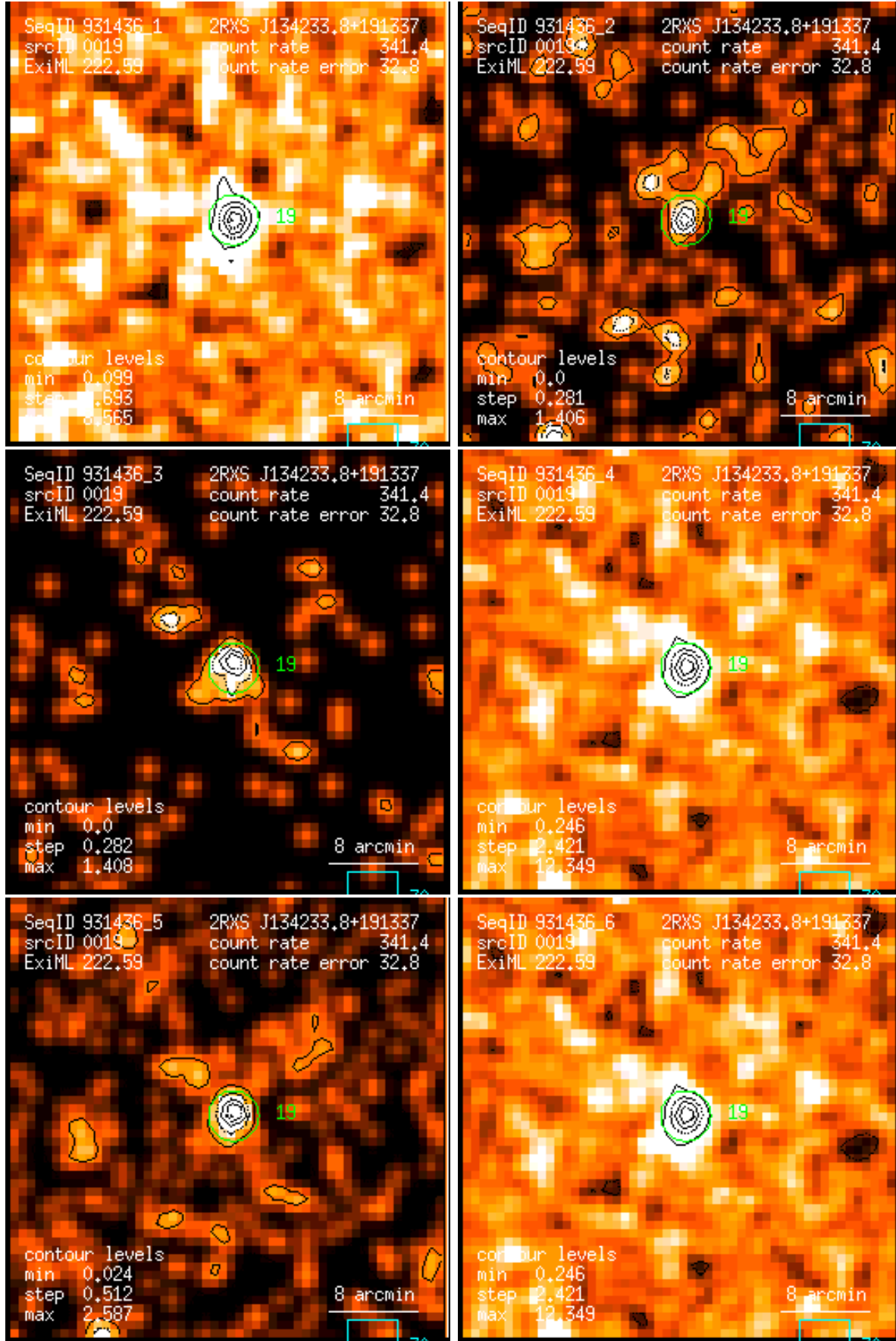
Figure 19: RASS 931436: detection 0019: band rate images, Gaussian filter: (1) PSPC channels 11 – 41, (2) 52 – 90, (3) 91 – 201, (4) 11 – 235, (5) 52 – 201, (6) 11 – 201. Broad band rates in counts/ks. Band rate contour levels in counts/ks/arcmin 2 .
