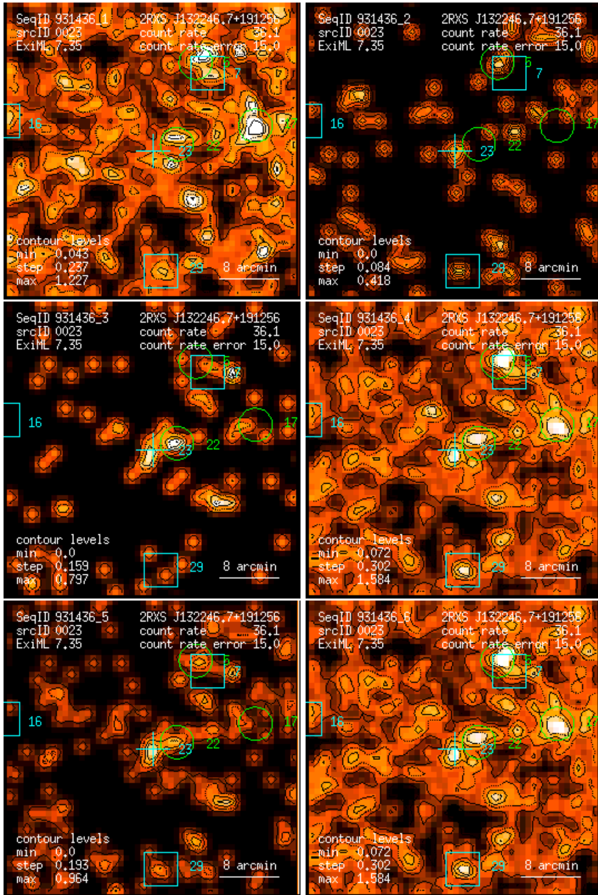
Figure 23: RASS 931436: detection 0023: band rate images, Gaussian filter: (1) PSPC channels 11 – 41, (2) 52 – 90, (3) 91 – 201, (4) 11 – 235, (5) 52 – 201, (6) 11 – 201. Broad band rates in counts/ks. Band rate contour levels in counts/ks/arcmin 2 .
