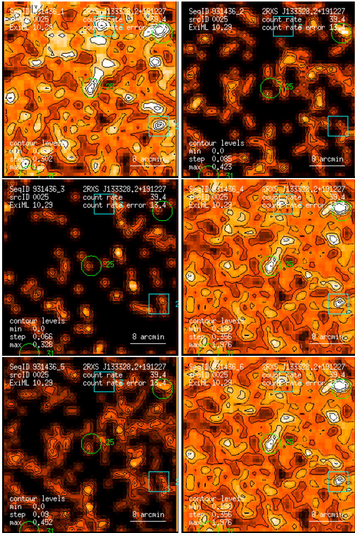
Figure 25: RASS 931436: detection 0025: band rate images, Gaussian filter: (1) PSPC channels 11 – 41, (2) 52 – 90, (3) 91 – 201, (4) 11 – 235, (5) 52 – 201, (6) 11 – 201. Broad band rates in counts/ks. Band rate contour levels in counts/ks/arcmin 2 .
