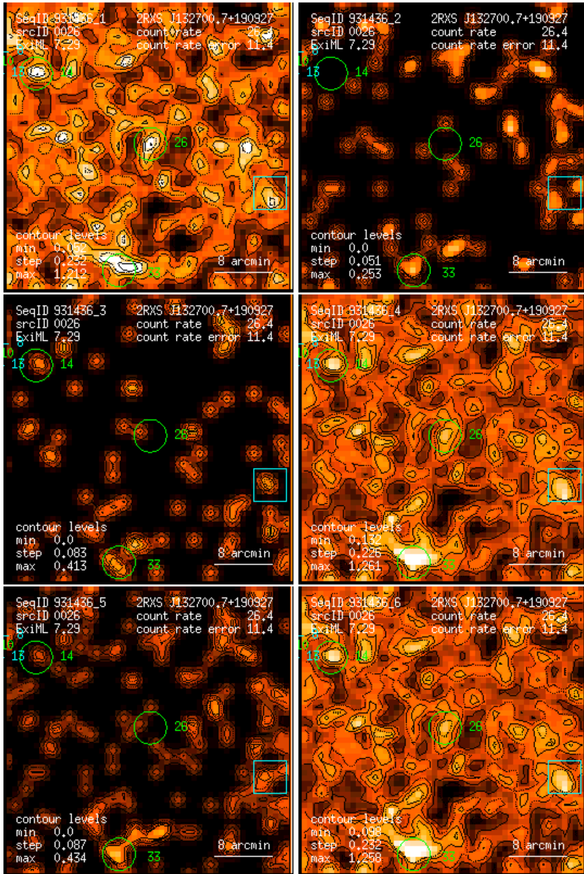
Figure 26: RASS 931436: detection 0026: band rate images, Gaussian filter: (1) PSPC channels 11 – 41, (2) 52 – 90, (3) 91 – 201, (4) 11 – 235, (5) 52 – 201, (6) 11 – 201. Broad band rates in counts/ks. Band rate contour levels in counts/ks/arcmin 2 .
