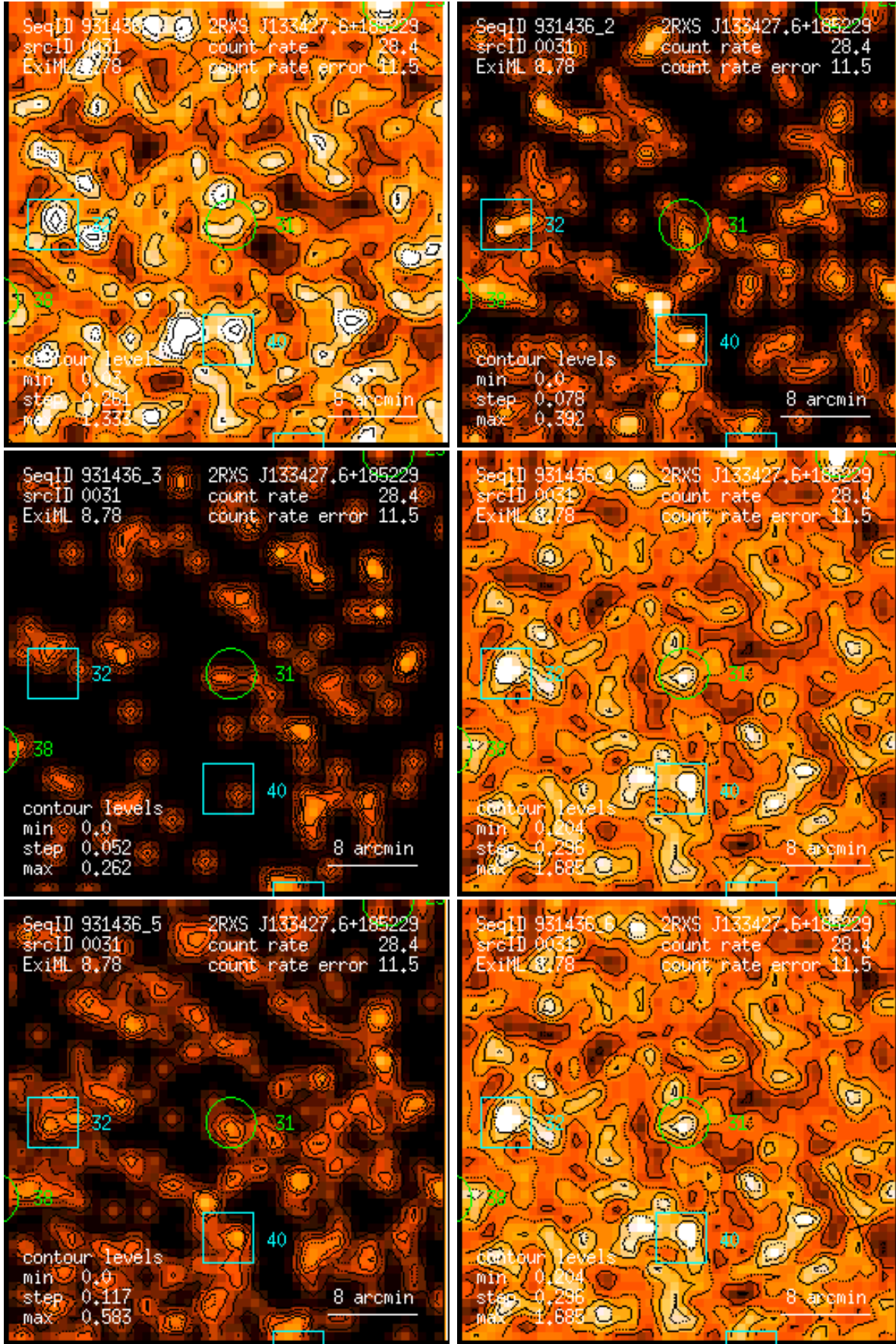
Figure 31: RASS 931436: detection 0031: band rate images, Gaussian filter: (1) PSPC channels 11 – 41, (2) 52 – 90, (3) 91 – 201, (4) 11 – 235, (5) 52 – 201, (6) 11 – 201. Broad band rates in counts/ks. Band rate contour levels in counts/ks/arcmin 2 .
