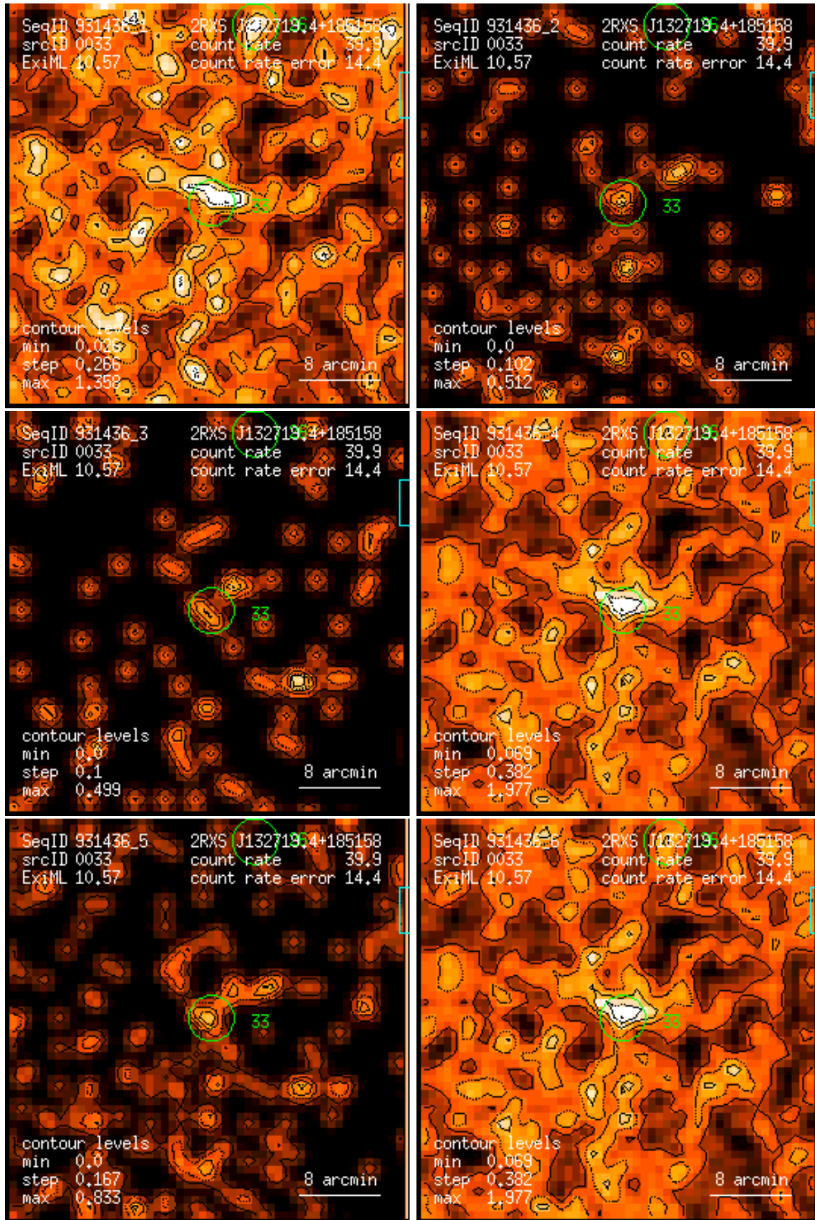
Figure 33: RASS 931436: detection 0033: band rate images, Gaussian filter: (1) PSPC channels 11 – 41, (2) 52 – 90, (3) 91 – 201, (4) 11 – 235, (5) 52 – 201, (6) 11 – 201. Broad band rates in counts/ks. Band rate contour levels in counts/ks/arcmin 2 .
