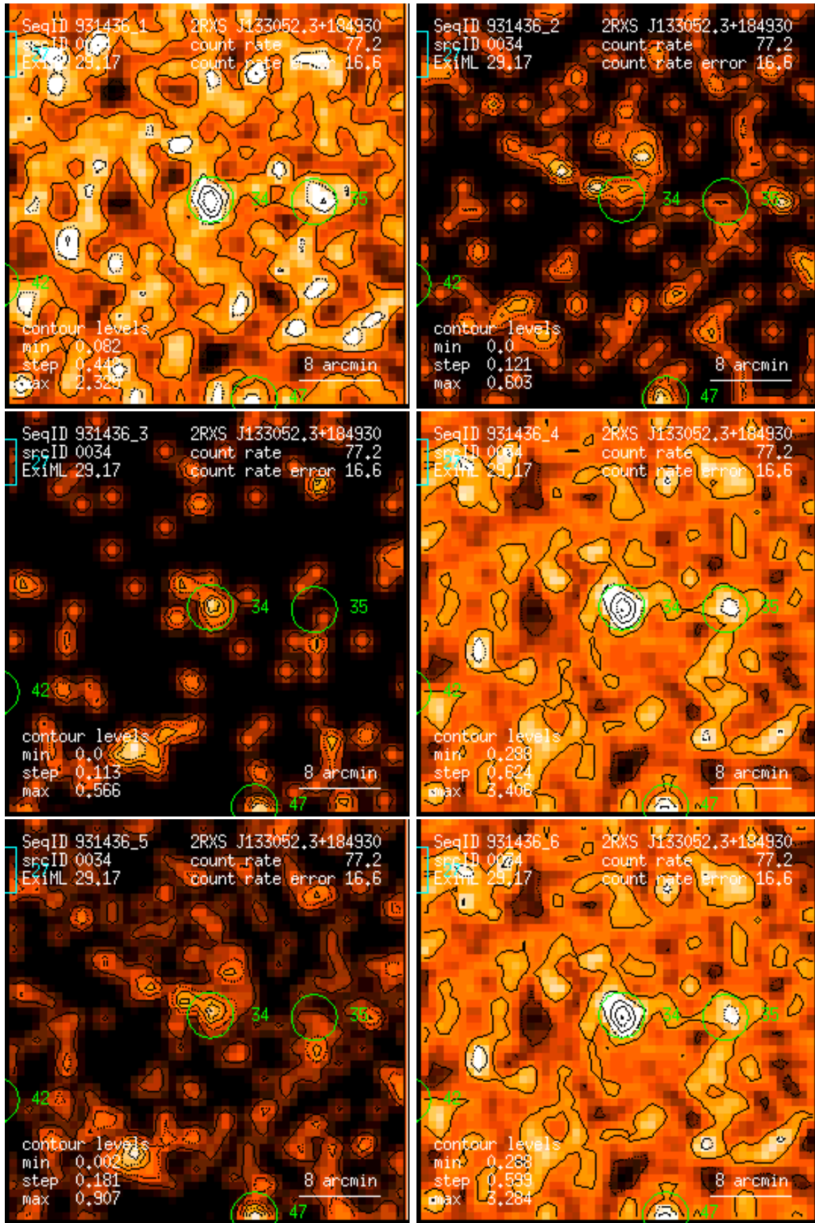
Figure 34: RASS 931436: detection 0034: band rate images, Gaussian filter: (1) PSPC channels 11 – 41, (2) 52 – 90, (3) 91 – 201, (4) 11 – 235, (5) 52 – 201, (6) 11 – 201. Broad band rates in counts/ks. Band rate contour levels in counts/ks/arcmin 2 .
