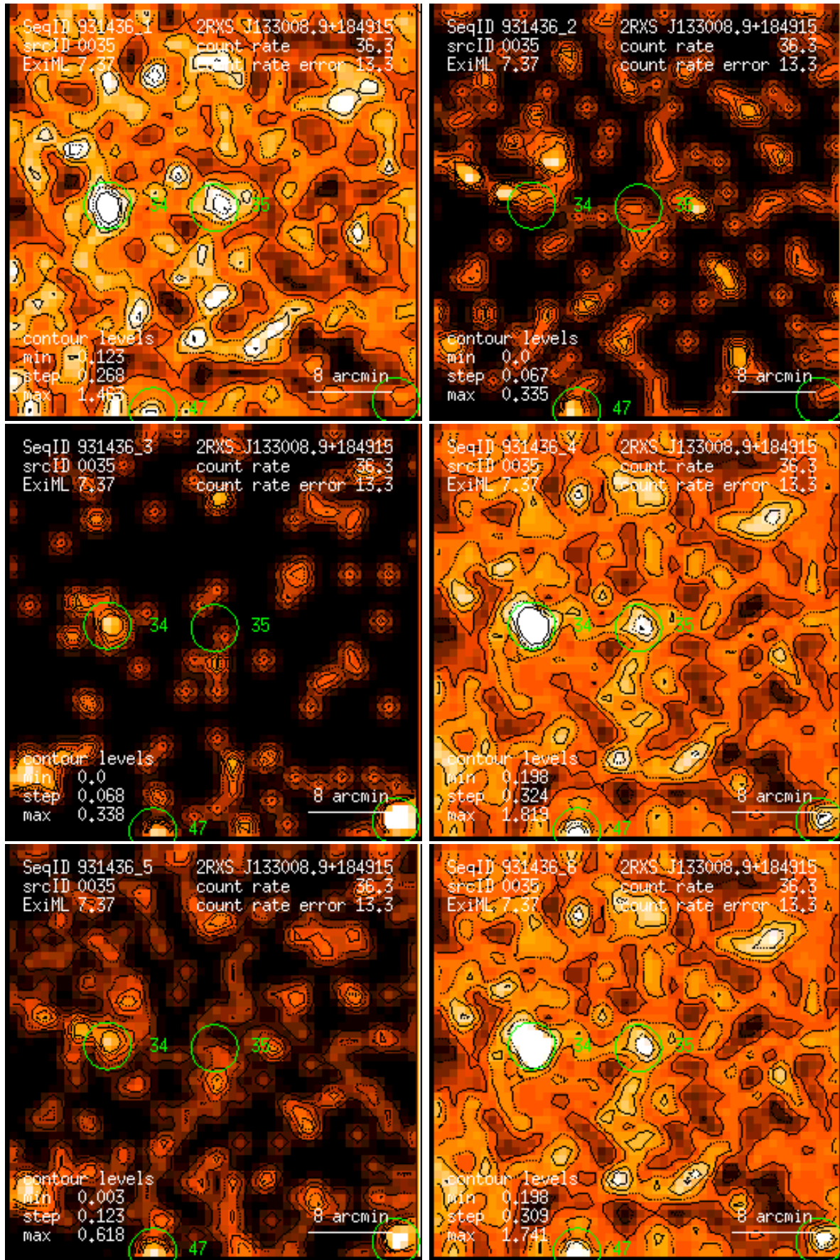
Figure 35: RASS 931436: detection 0035: band rate images, Gaussian filter: (1) PSPC channels 11 – 41, (2) 52 – 90, (3) 91 – 201, (4) 11 – 235, (5) 52 – 201, (6) 11 – 201. Broad band rates in counts/ks. Band rate contour levels in counts/ks/arcmin 2 .
