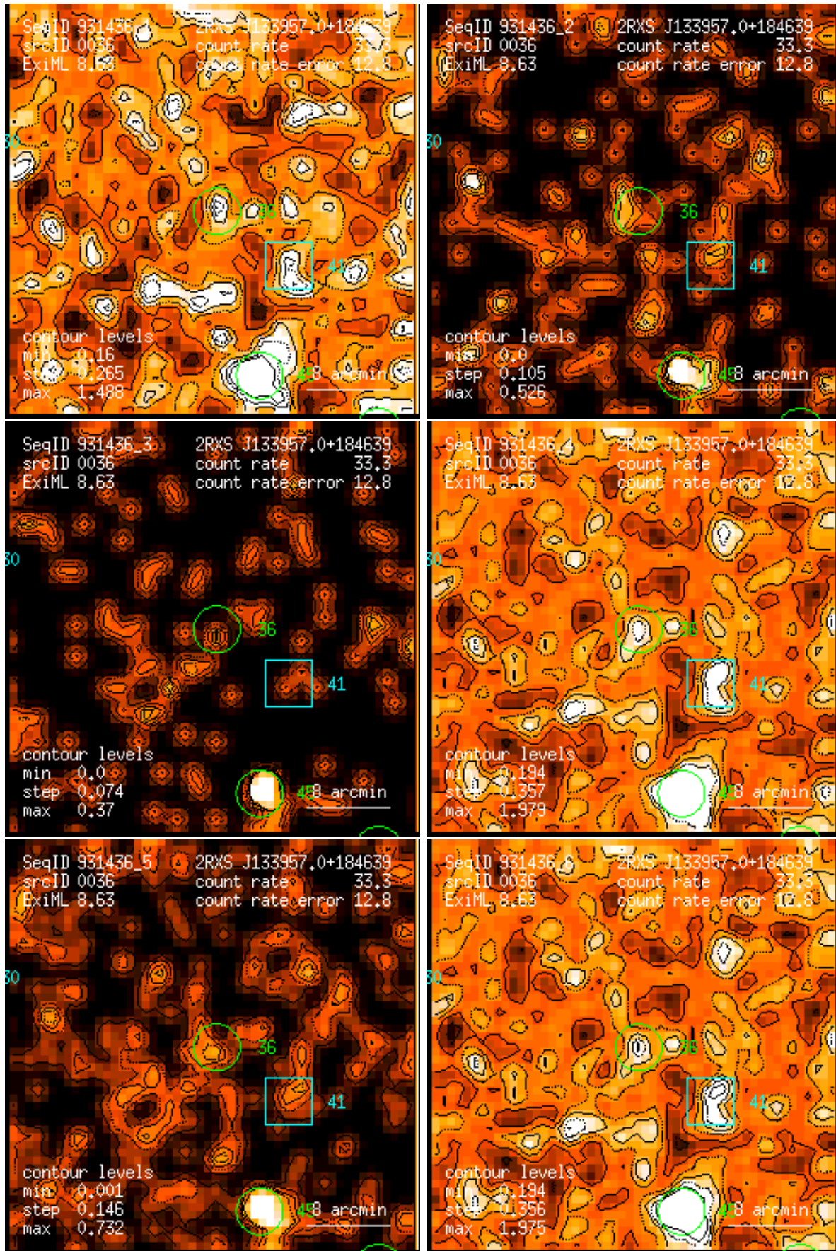
Figure 36: RASS 931436: detection 0036: band rate images, Gaussian filter: (1) PSPC channels 11 – 41, (2) 52 – 90, (3) 91 – 201, (4) 11 – 235, (5) 52 – 201, (6) 11 – 201. Broad band rates in counts/ks. Band rate contour levels in counts/ks/arcmin 2 .
