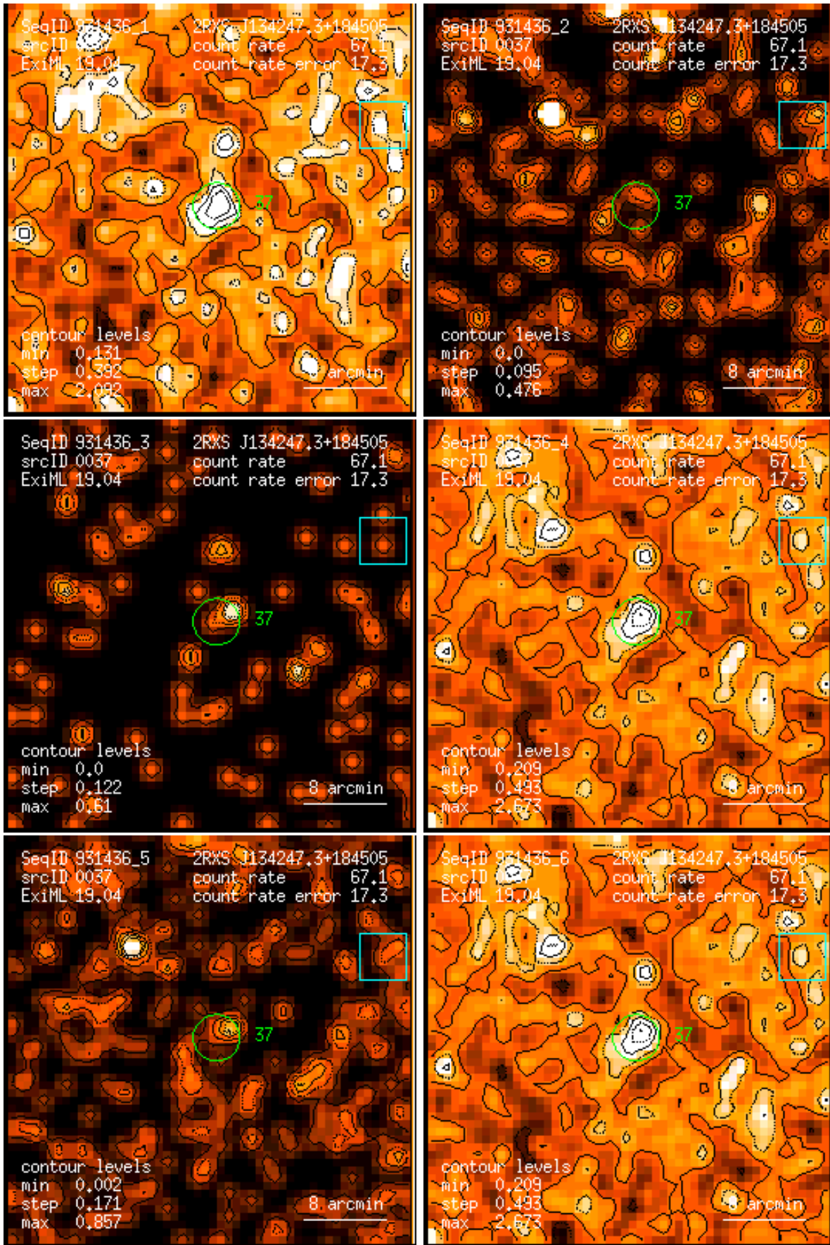
Figure 37: RASS 931436: detection 0037: band rate images, Gaussian filter: (1) PSPC channels 11 – 41, (2) 52 – 90, (3) 91 – 201, (4) 11 – 235, (5) 52 – 201, (6) 11 – 201. Broad band rates in counts/ks. Band rate contour levels in counts/ks/arcmin 2 .
