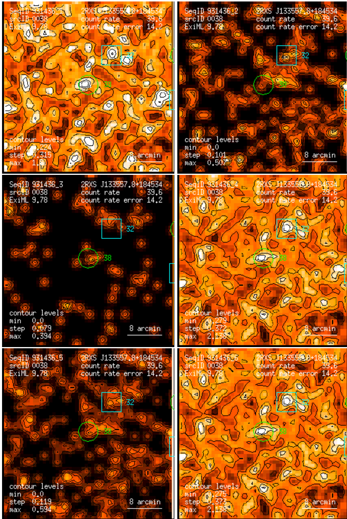
Figure 38: RASS 931436: detection 0038: band rate images, Gaussian filter: (1) PSPC channels 11 – 41, (2) 52 – 90, (3) 91 – 201, (4) 11 – 235, (5) 52 – 201, (6) 11 – 201. Broad band rates in counts/ks. Band rate contour levels in counts/ks/arcmin 2 .
