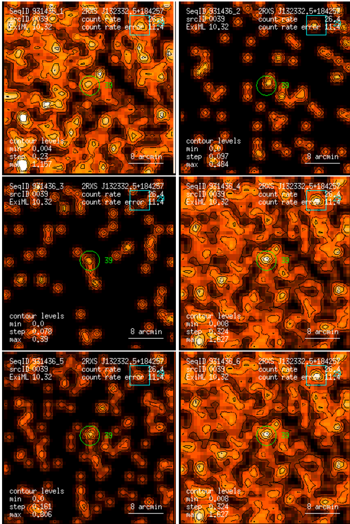
Figure 39: RASS 931436: detection 0039: band rate images, Gaussian filter: (1) PSPC channels 11 – 41, (2) 52 – 90, (3) 91 – 201, (4) 11 – 235, (5) 52 – 201, (6) 11 – 201. Broad band rates in counts/ks. Band rate contour levels in counts/ks/arcmin 2 .
