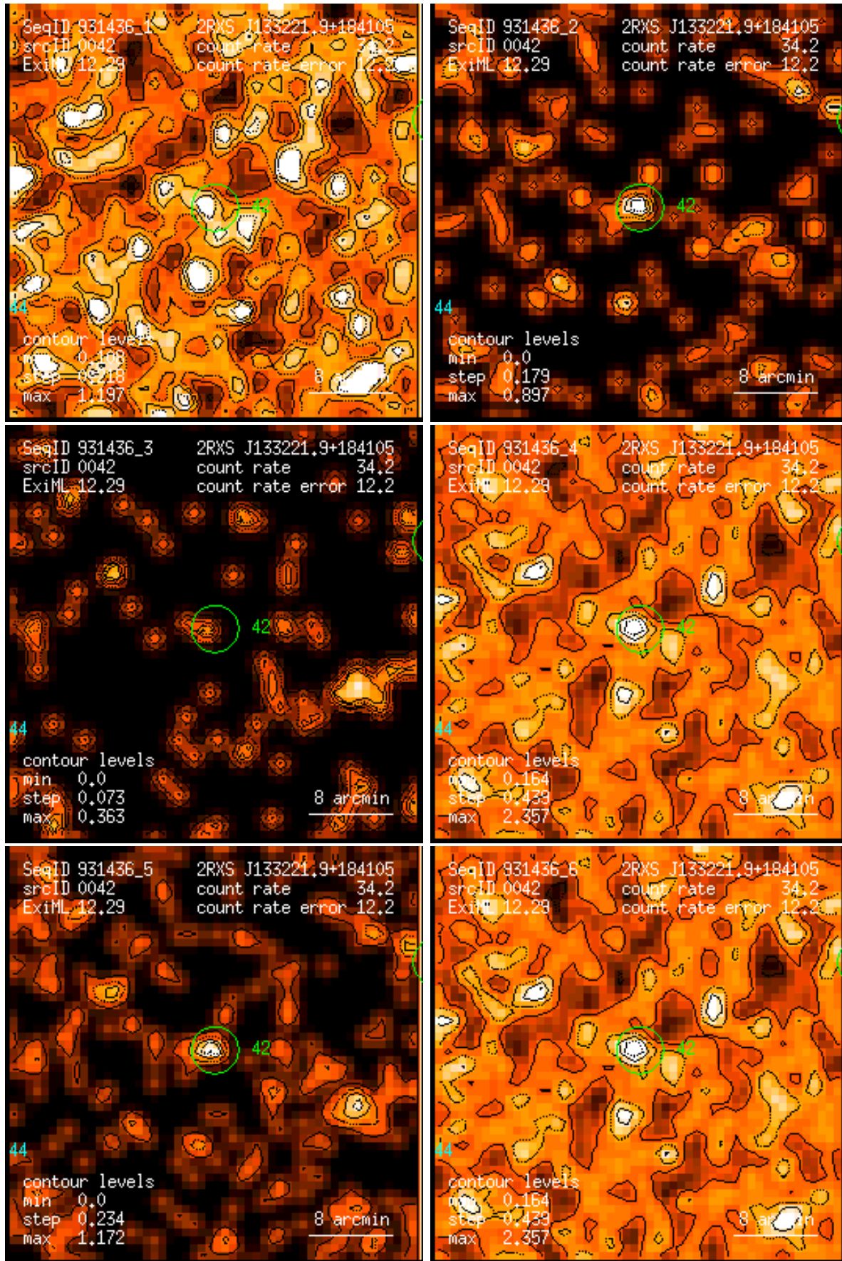
Figure 42: RASS 931436: detection 0042: band rate images, Gaussian filter: (1) PSPC channels 11 – 41, (2) 52 – 90, (3) 91 – 201, (4) 11 – 235, (5) 52 – 201, (6) 11 – 201. Broad band rates in counts/ks. Band rate contour levels in counts/ks/arcmin 2 .
