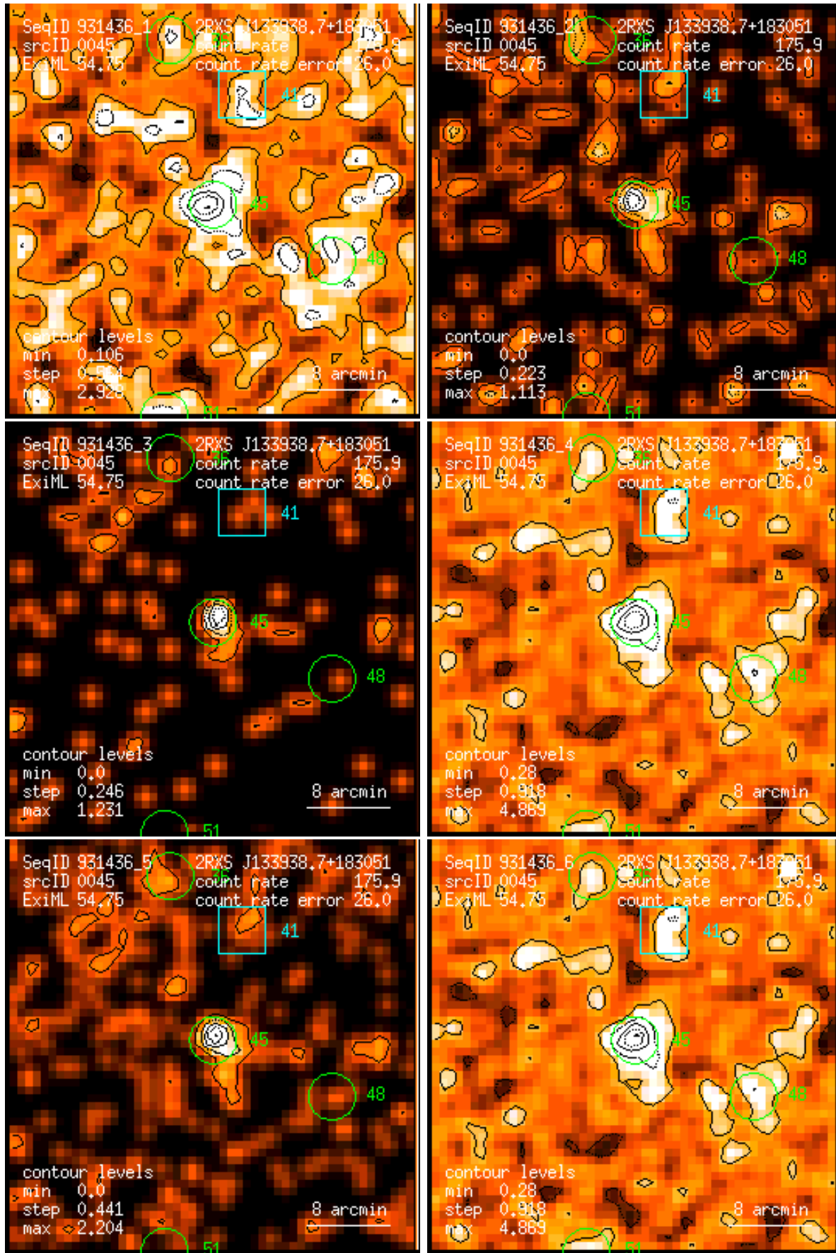
Figure 45: RASS 931436: detection 0045: band rate images, Gaussian filter: (1) PSPC channels 11 – 41, (2) 52 – 90, (3) 91 – 201, (4) 11 – 235, (5) 52 – 201, (6) 11 – 201. Broad band rates in counts/ks. Band rate contour levels in counts/ks/arcmin 2 .
