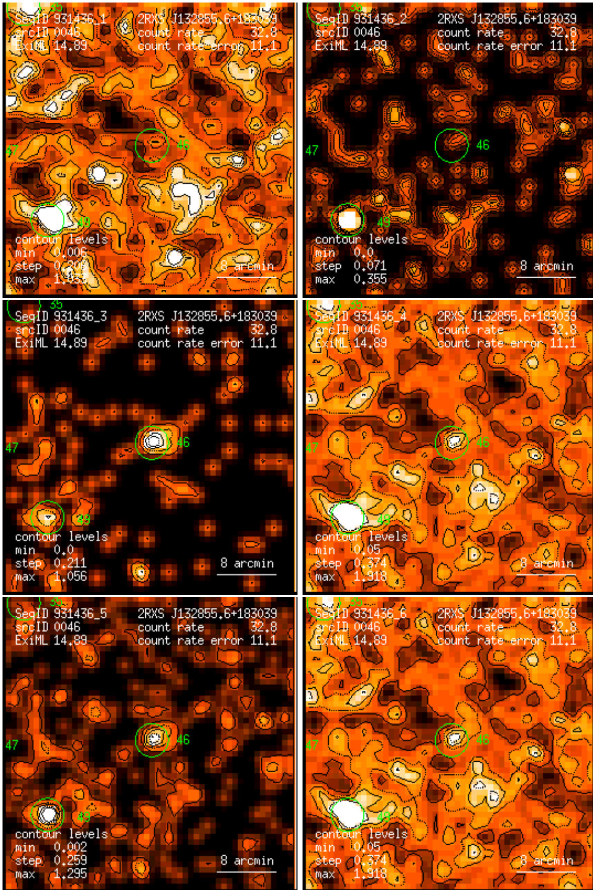
Figure 46: RASS 931436: detection 0046: band rate images, Gaussian filter: (1) PSPC channels 11 – 41, (2) 52 – 90, (3) 91 – 201, (4) 11 – 235, (5) 52 – 201, (6) 11 – 201. Broad band rates in counts/ks. Band rate contour levels in counts/ks/arcmin 2 .
