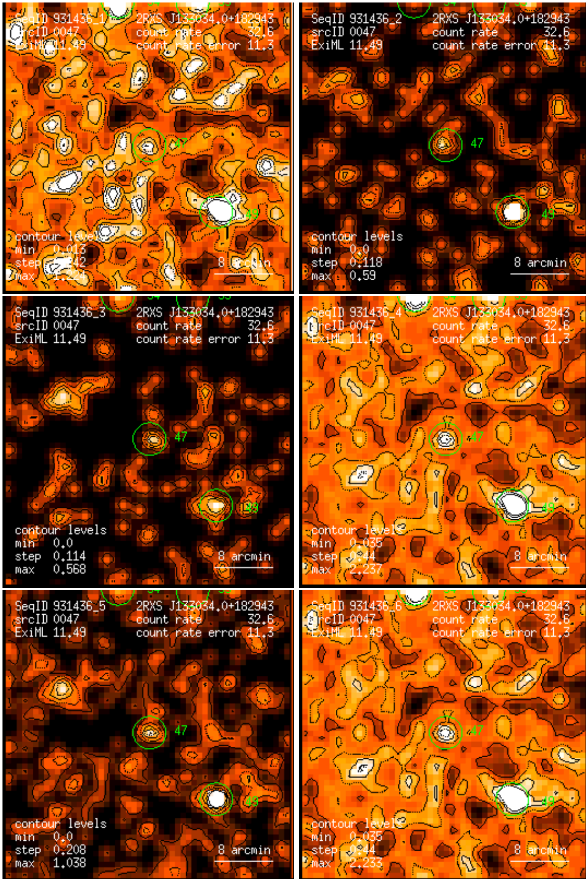
Figure 47: RASS 931436: detection 0047: band rate images, Gaussian filter: (1) PSPC channels 11 – 41, (2) 52 – 90, (3) 91 – 201, (4) 11 – 235, (5) 52 – 201, (6) 11 – 201. Broad band rates in counts/ks. Band rate contour levels in counts/ks/arcmin 2 .
