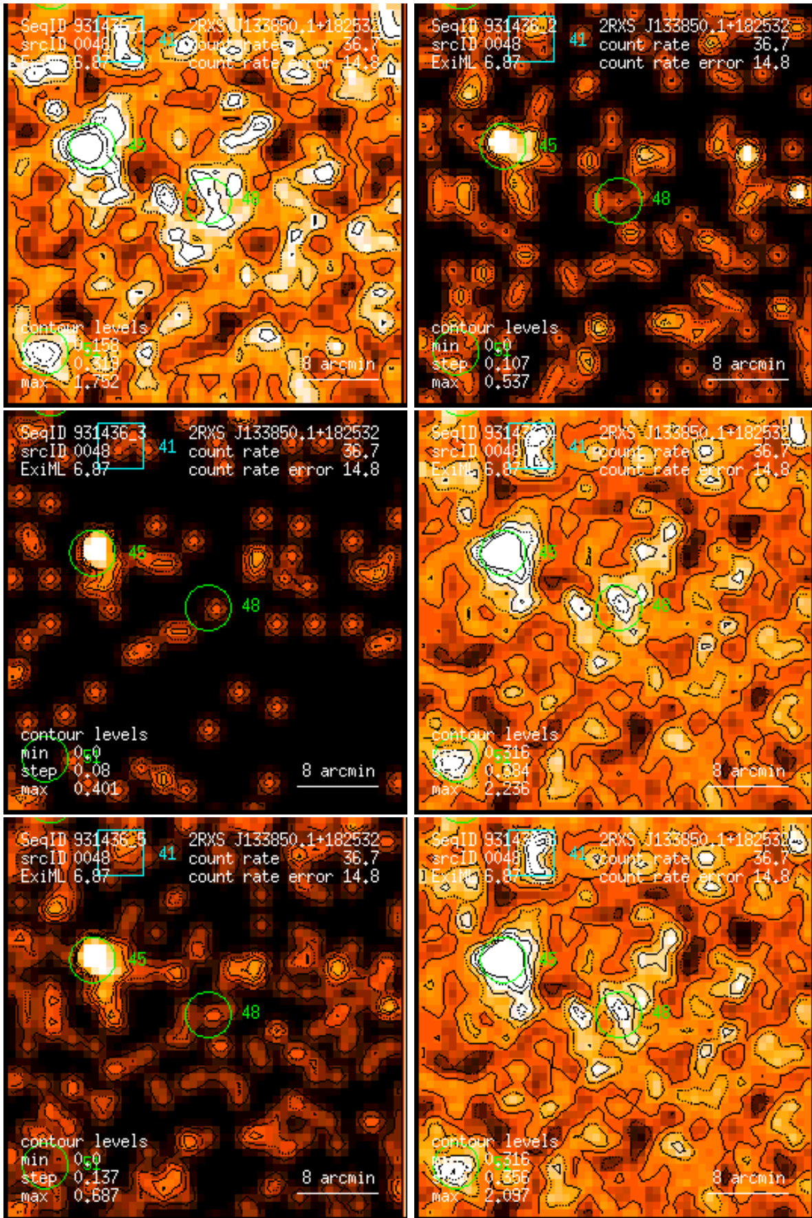
Figure 48: RASS 931436: detection 0048: band rate images, Gaussian filter: (1) PSPC channels 11 – 41, (2) 52 – 90, (3) 91 – 201, (4) 11 – 235, (5) 52 – 201, (6) 11 – 201. Broad band rates in counts/ks. Band rate contour levels in counts/ks/arcmin 2 .
