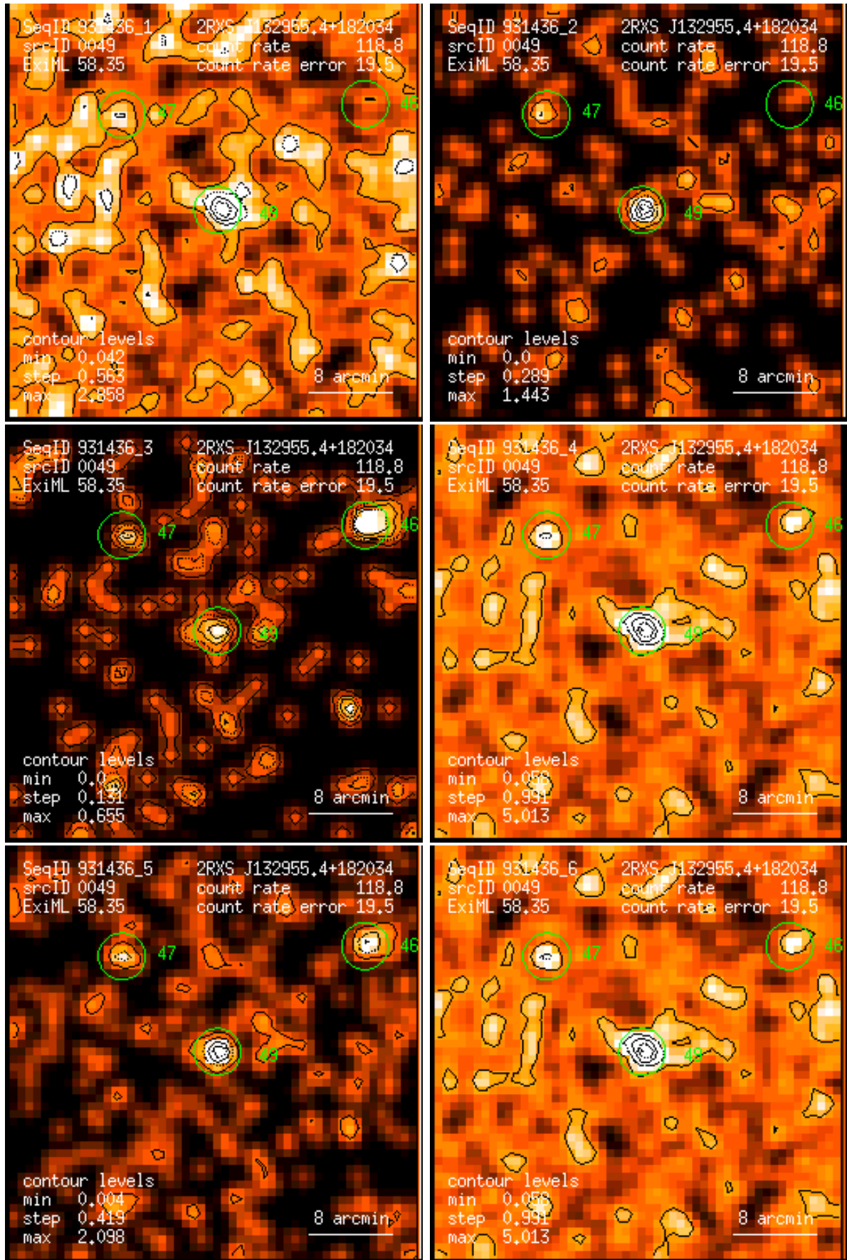
Figure 49: RASS 931436: detection 0049: band rate images, Gaussian filter: (1) PSPC channels 11 – 41, (2) 52 – 90, (3) 91 – 201, (4) 11 – 235, (5) 52 – 201, (6) 11 – 201. Broad band rates in counts/ks. Band rate contour levels in counts/ks/arcmin 2 .
