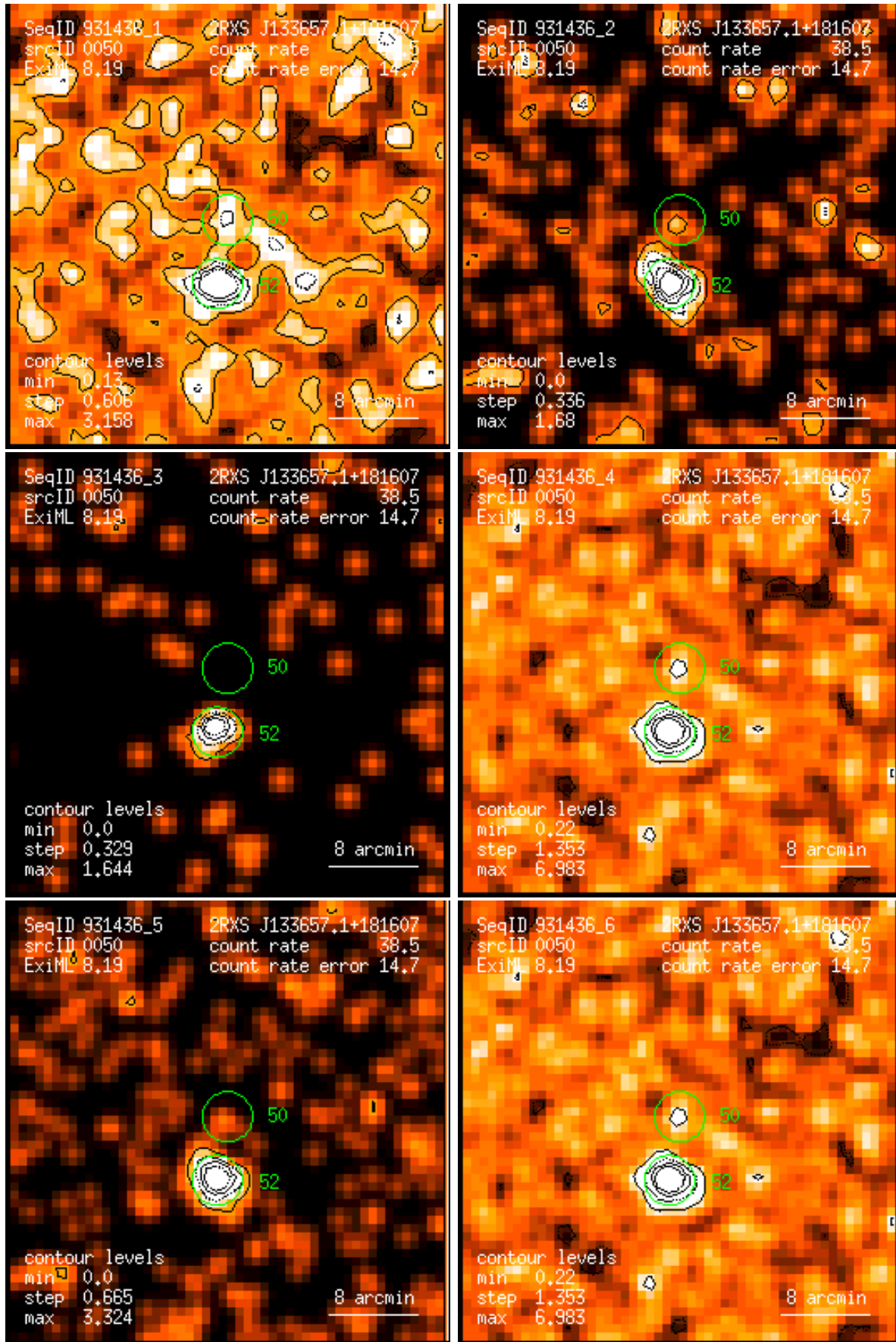
Figure 50: RASS 931436: detection 0050: band rate images, Gaussian filter: (1) PSPC channels 11 – 41, (2) 52 – 90, (3) 91 – 201, (4) 11 – 235, (5) 52 – 201, (6) 11 – 201. Broad band rates in counts/ks. Band rate contour levels in counts/ks/arcmin 2 .
