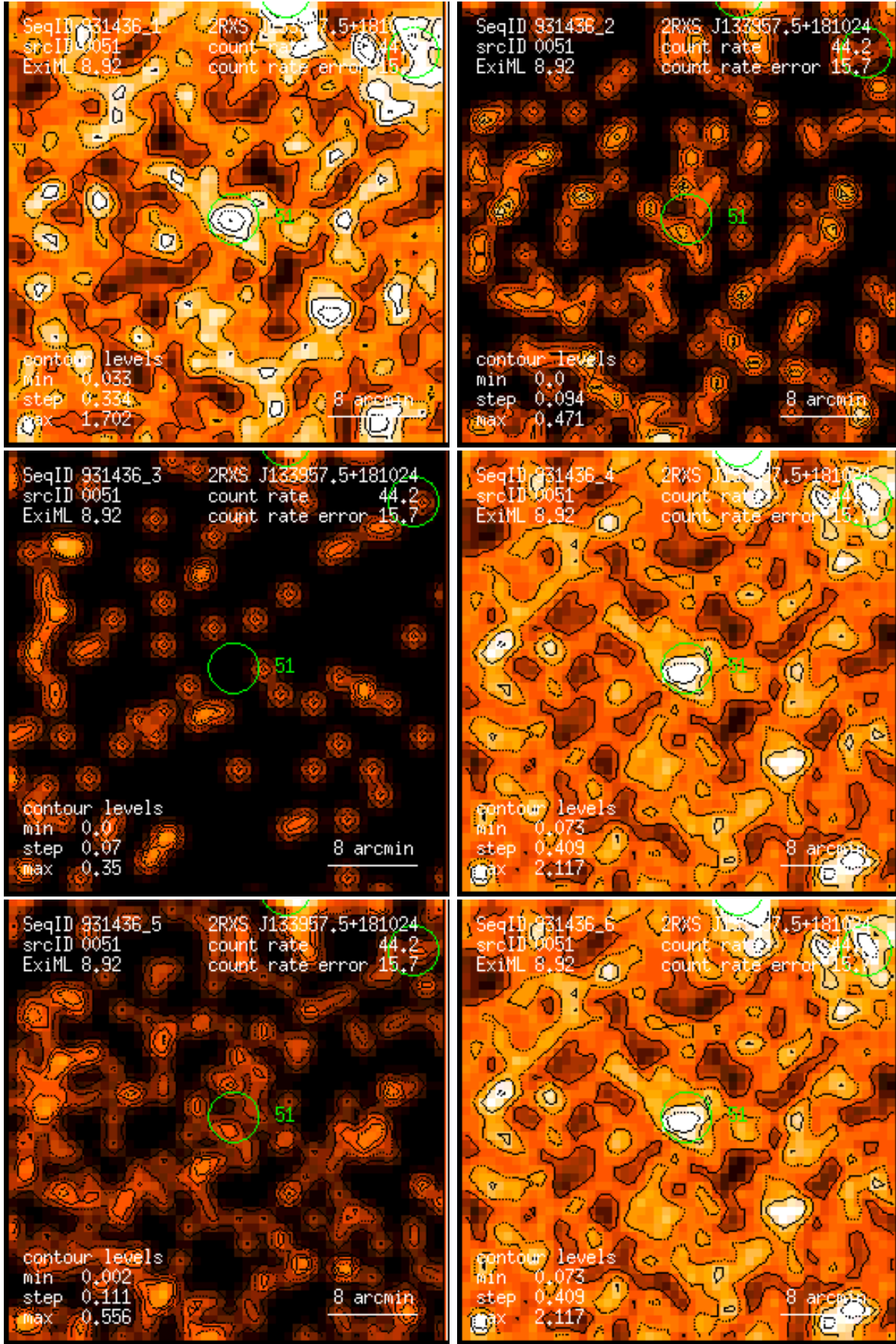
Figure 51: RASS 931436: detection 0051: band rate images, Gaussian filter: (1) PSPC channels 11 – 41, (2) 52 – 90, (3) 91 – 201, (4) 11 – 235, (5) 52 – 201, (6) 11 – 201. Broad band rates in counts/ks. Band rate contour levels in counts/ks/arcmin 2 .
