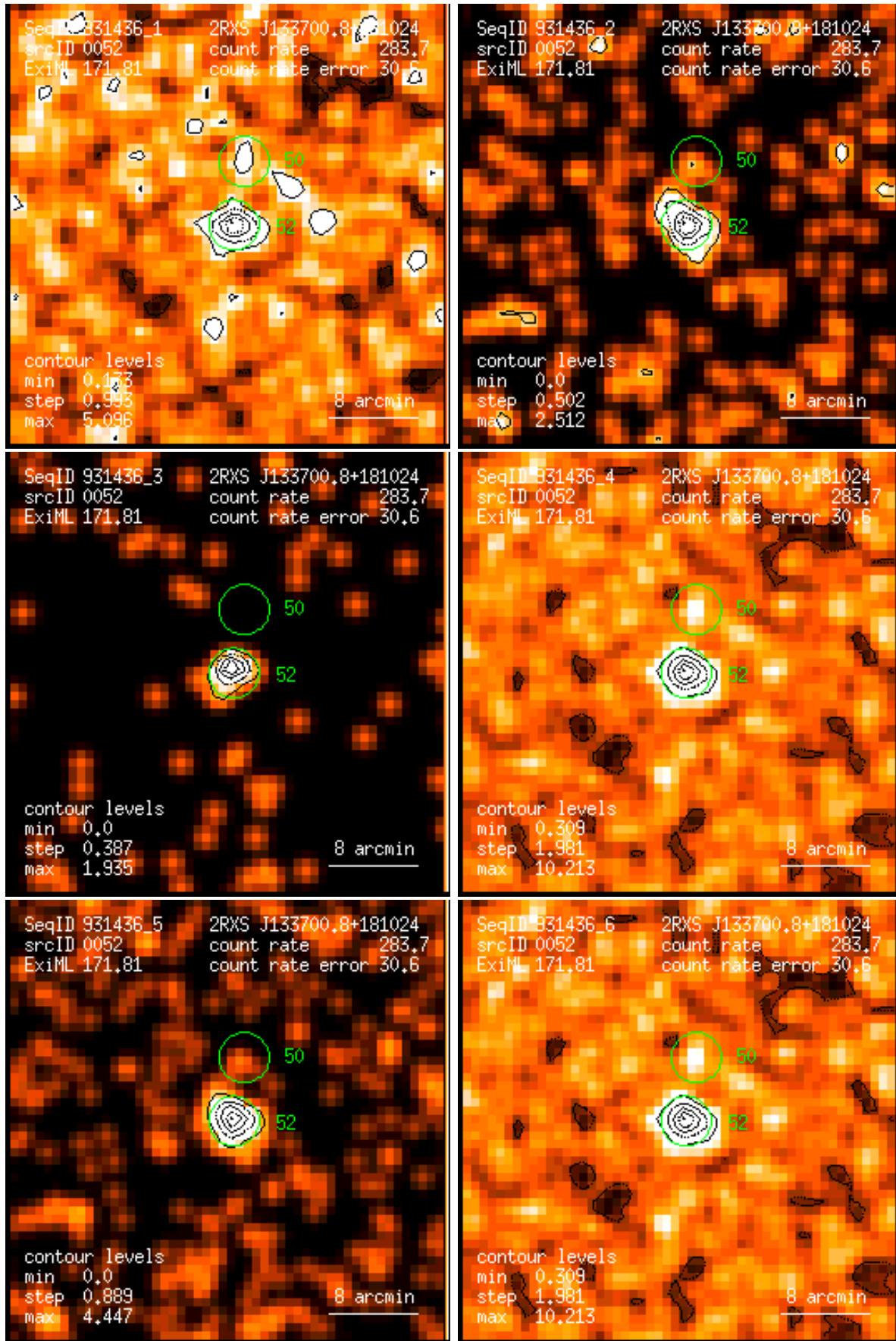
Figure 52: RASS 931436: detection 0052: band rate images, Gaussian filter: (1) PSPC channels 11 – 41, (2) 52 – 90, (3) 91 – 201, (4) 11 – 235, (5) 52 – 201, (6) 11 – 201. Broad band rates in counts/ks. Band rate contour levels in counts/ks/arcmin 2 .
