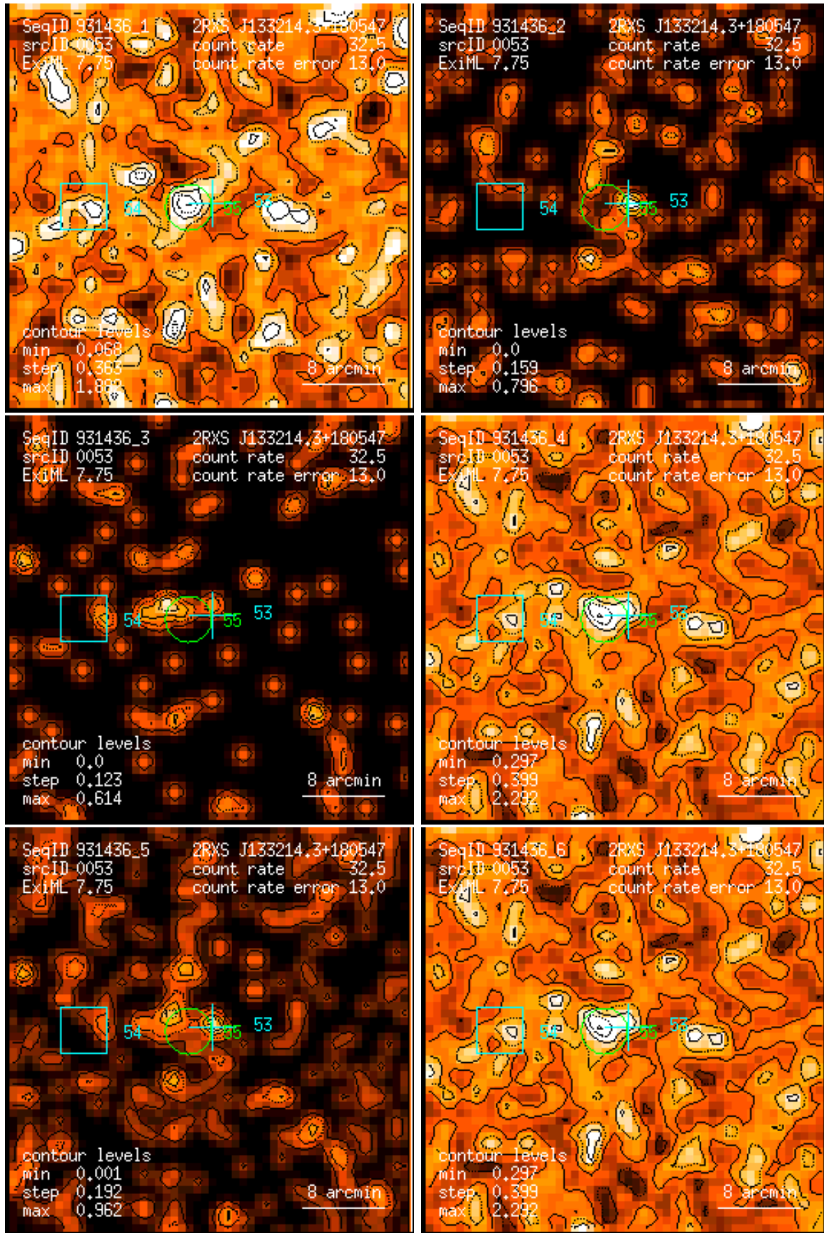
Figure 53: RASS 931436: detection 0053: band rate images, Gaussian filter: (1) PSPC channels 11 – 41, (2) 52 – 90, (3) 91 – 201, (4) 11 – 235, (5) 52 – 201, (6) 11 – 201. Broad band rates in counts/ks. Band rate contour levels in counts/ks/arcmin 2 .
