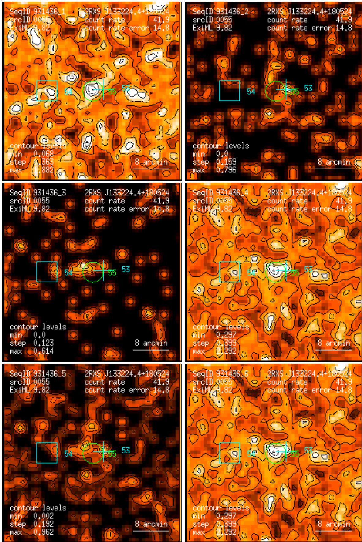
Figure 55: RASS 931436: detection 0055: band rate images, Gaussian filter: (1) PSPC channels 11 – 41, (2) 52 – 90, (3) 91 – 201, (4) 11 – 235, (5) 52 – 201, (6) 11 – 201. Broad band rates in counts/ks. Band rate contour levels in counts/ks/arcmin 2 .
