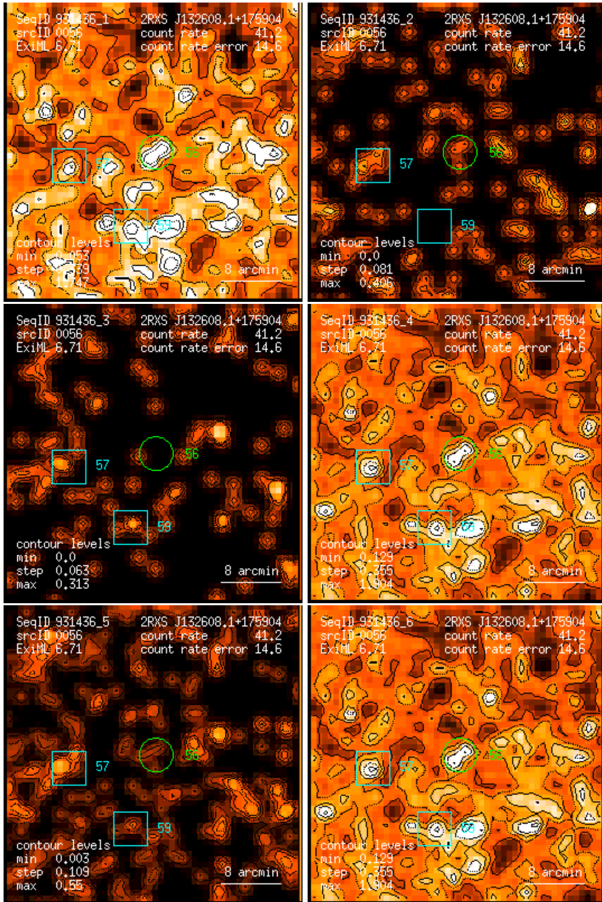
Figure 56: RASS 931436: detection 0056: band rate images, Gaussian filter: (1) PSPC channels 11 – 41, (2) 52 – 90, (3) 91 – 201, (4) 11 – 235, (5) 52 – 201, (6) 11 – 201. Broad band rates in counts/ks. Band rate contour levels in counts/ks/arcmin 2 .
