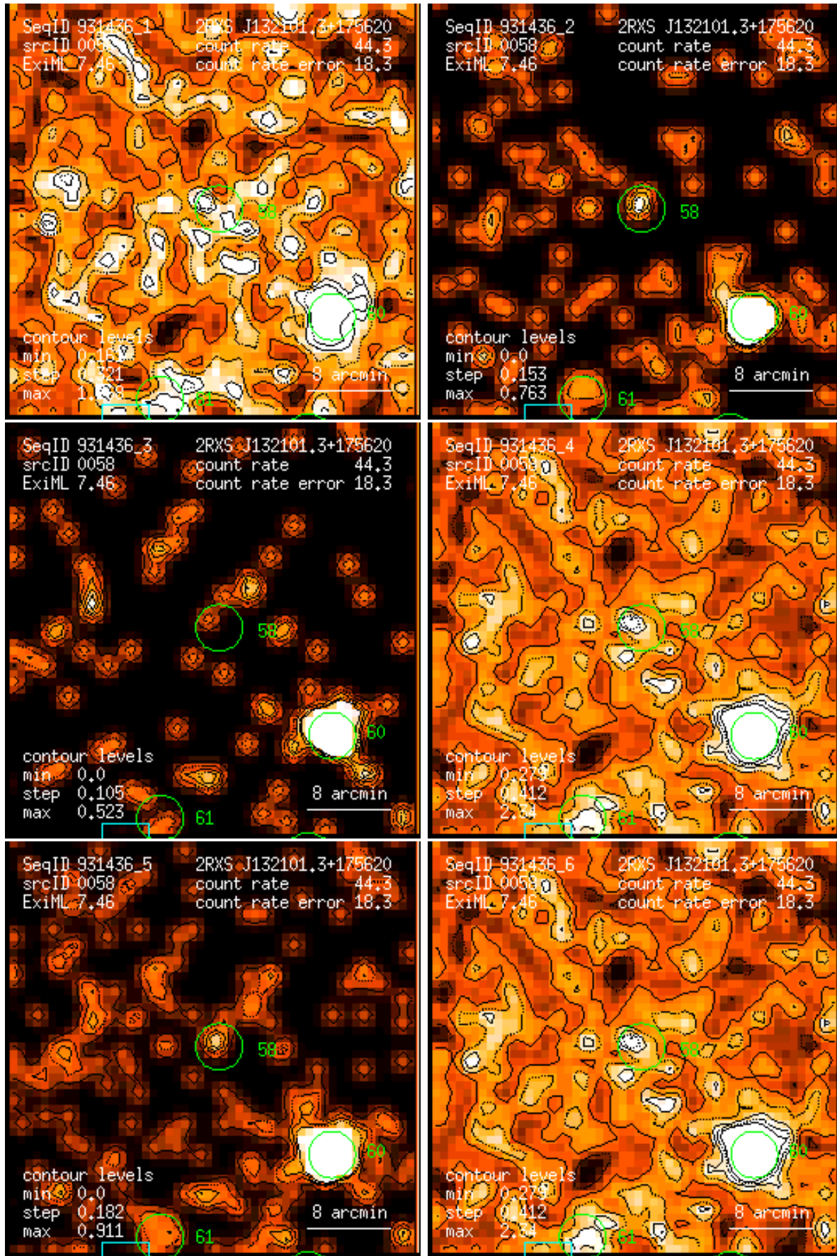
Figure 58: RASS 931436: detection 0058: band rate images, Gaussian filter: (1) PSPC channels 11 – 41, (2) 52 – 90, (3) 91 – 201, (4) 11 – 235, (5) 52 – 201, (6) 11 – 201. Broad band rates in counts/ks. Band rate contour levels in counts/ks/arcmin 2 .
