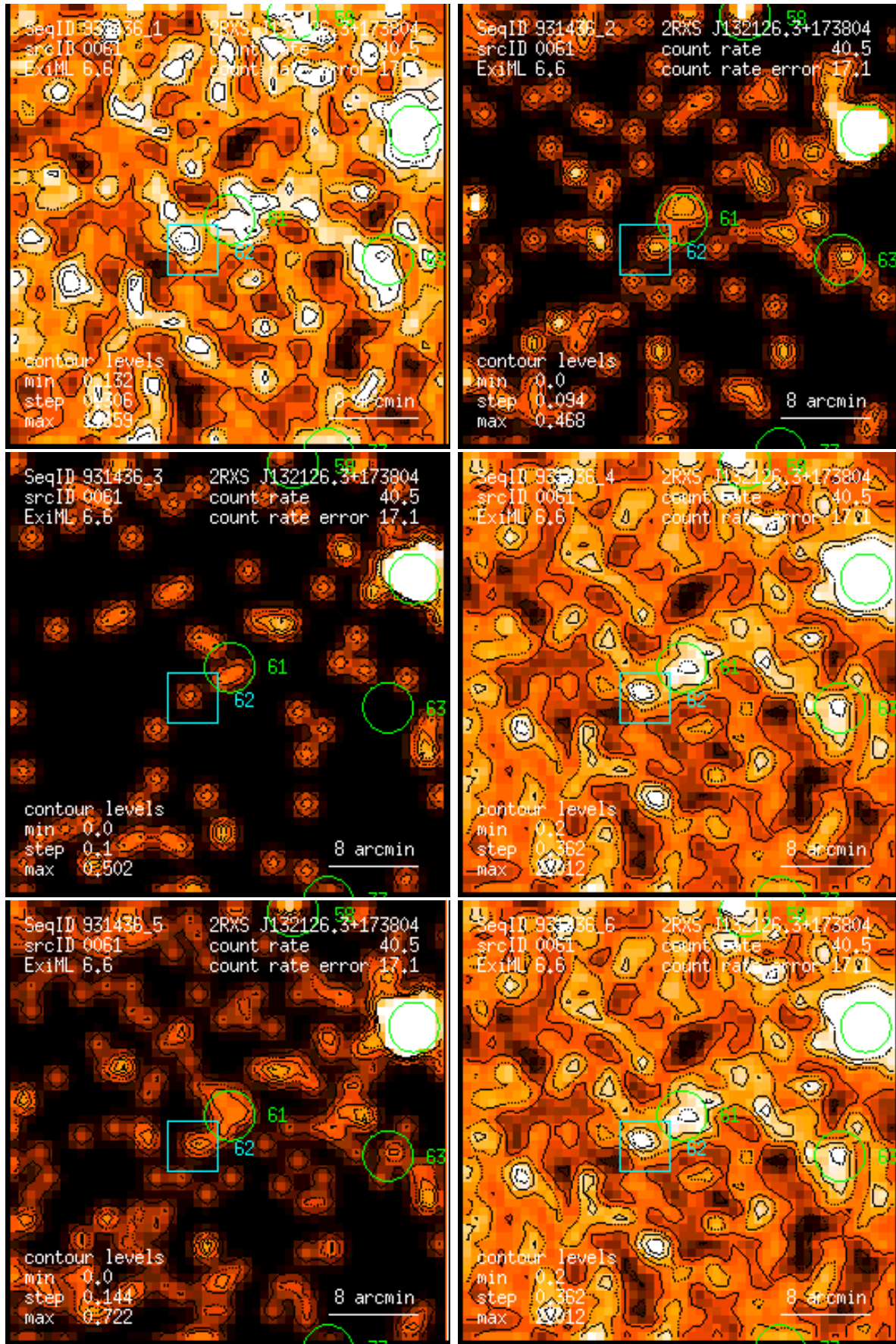
Figure 61: RASS 931436: detection 0061: band rate images, Gaussian filter: (1) PSPC channels 11 – 41, (2) 52 – 90, (3) 91 – 201, (4) 11 – 235, (5) 52 – 201, (6) 11 – 201. Broad band rates in counts/ks. Band rate contour levels in counts/ks/arcmin 2 .
