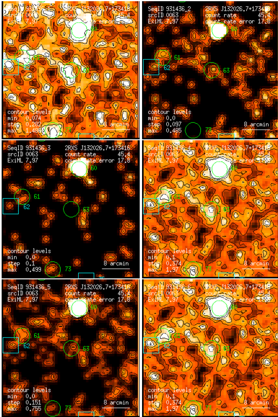
Figure 63: RASS 931436: detection 0063: band rate images, Gaussian filter: (1) PSPC channels 11 – 41, (2) 52 – 90, (3) 91 – 201, (4) 11 – 235, (5) 52 – 201, (6) 11 – 201. Broad band rates in counts/ks. Band rate contour levels in counts/ks/arcmin 2 .
