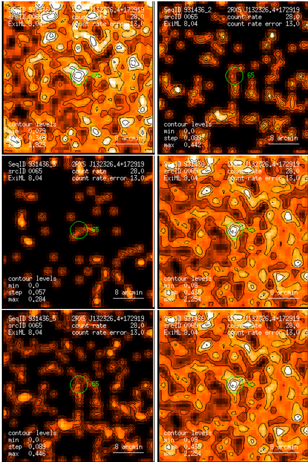
Figure 65: RASS 931436: detection 0065: band rate images, Gaussian filter: (1) PSPC channels 11 – 41, (2) 52 – 90, (3) 91 – 201, (4) 11 – 235, (5) 52 – 201, (6) 11 – 201. Broad band rates in counts/ks. Band rate contour levels in counts/ks/arcmin 2 .
