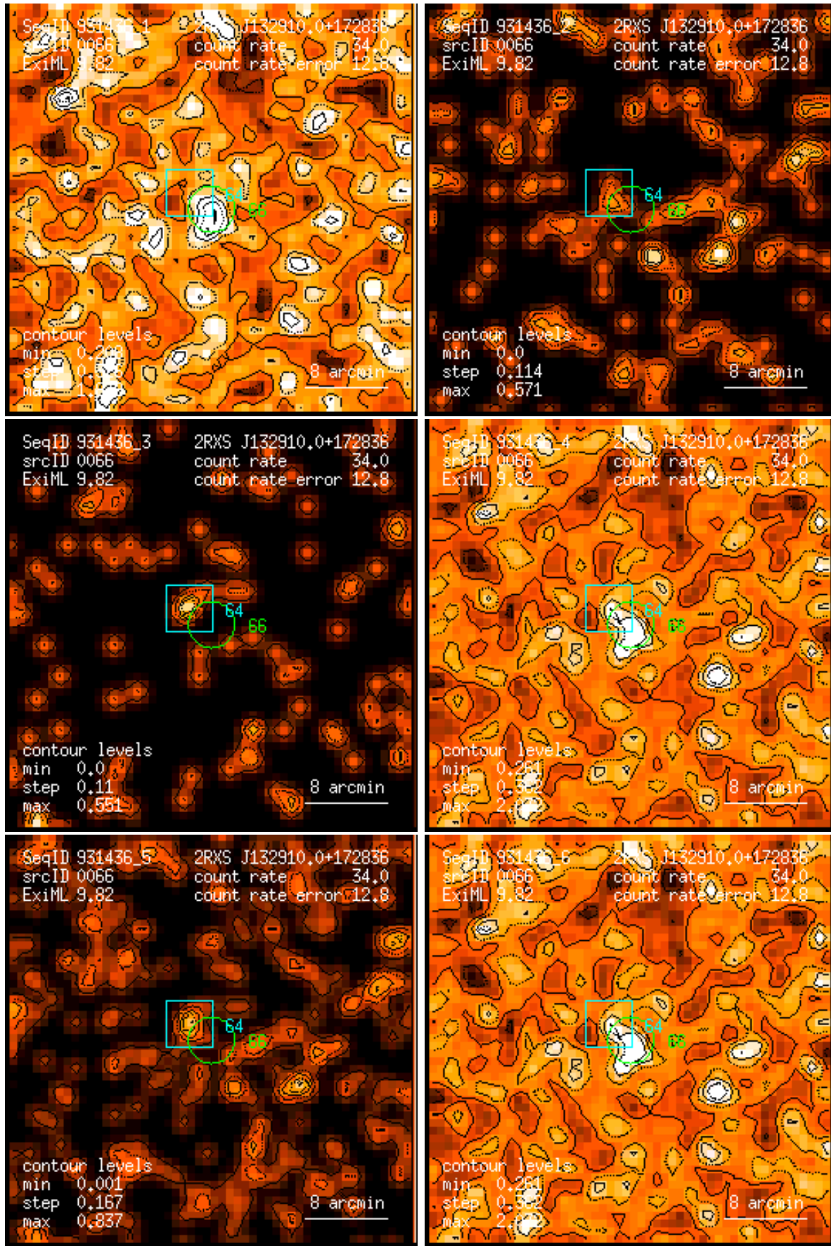
Figure 66: RASS 931436: detection 0066: band rate images, Gaussian filter: (1) PSPC channels 11 – 41, (2) 52 – 90, (3) 91 – 201, (4) 11 – 235, (5) 52 – 201, (6) 11 – 201. Broad band rates in counts/ks. Band rate contour levels in counts/ks/arcmin 2 .
