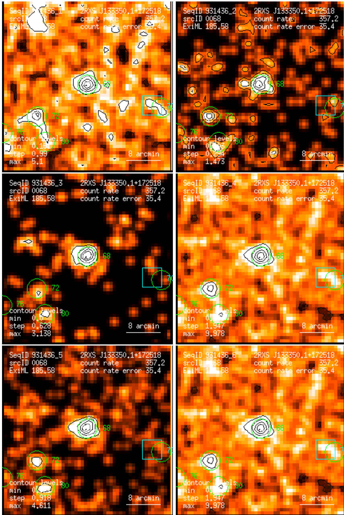
Figure 68: RASS 931436: detection 0068: band rate images, Gaussian filter: (1) PSPC channels 11 – 41, (2) 52 – 90, (3) 91 – 201, (4) 11 – 235, (5) 52 – 201, (6) 11 – 201. Broad band rates in counts/ks. Band rate contour levels in counts/ks/arcmin 2 .
