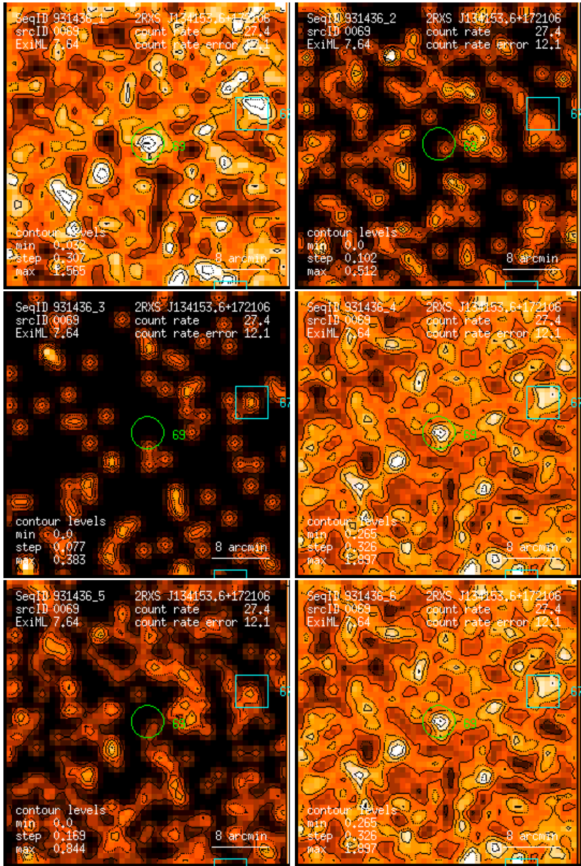
Figure 69: RASS 931436: detection 0069: band rate images, Gaussian filter: (1) PSPC channels 11 – 41, (2) 52 – 90, (3) 91 – 201, (4) 11 – 235, (5) 52 – 201, (6) 11 – 201. Broad band rates in counts/ks. Band rate contour levels in counts/ks/arcmin 2 .
