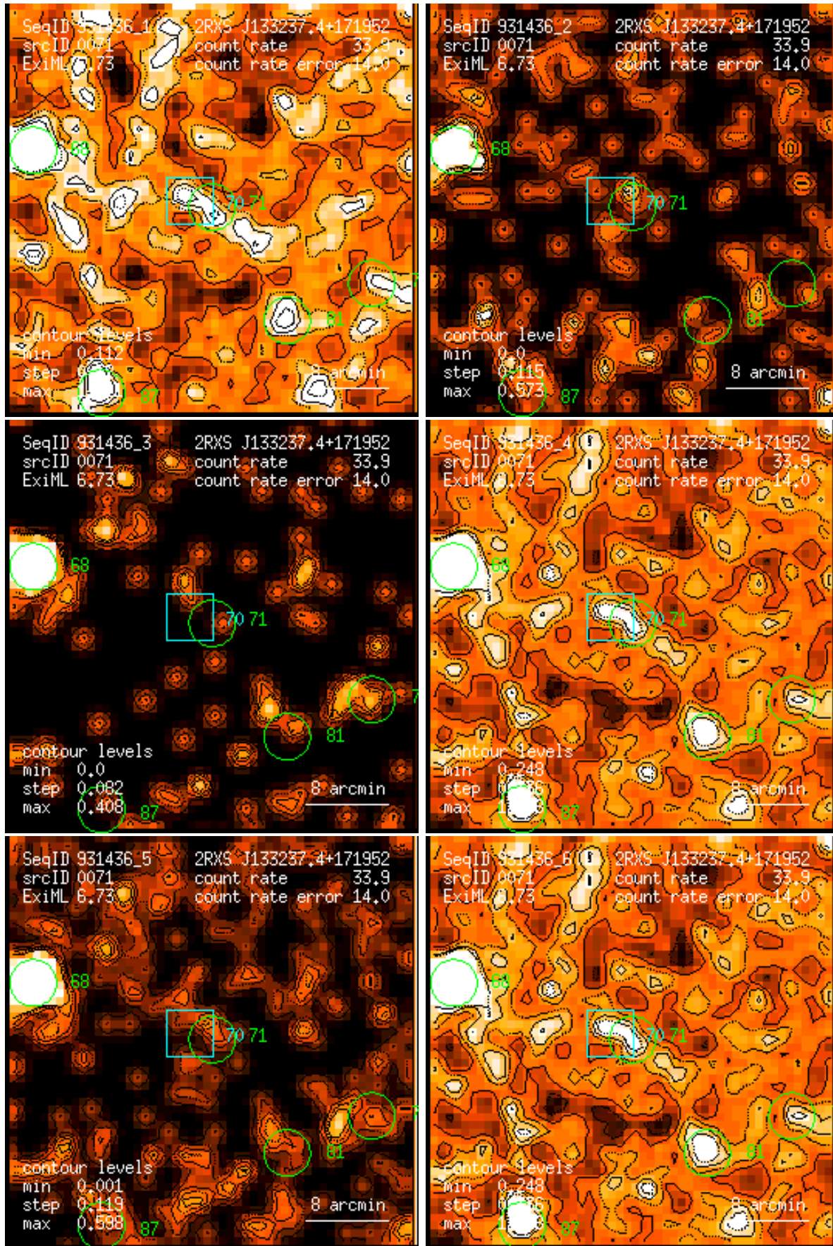
Figure 71: RASS 931436: detection 0071: band rate images, Gaussian filter: (1) PSPC channels 11 – 41, (2) 52 – 90, (3) 91 – 201, (4) 11 – 235, (5) 52 – 201, (6) 11 – 201. Broad band rates in counts/ks. Band rate contour levels in counts/ks/arcmin 2 .
