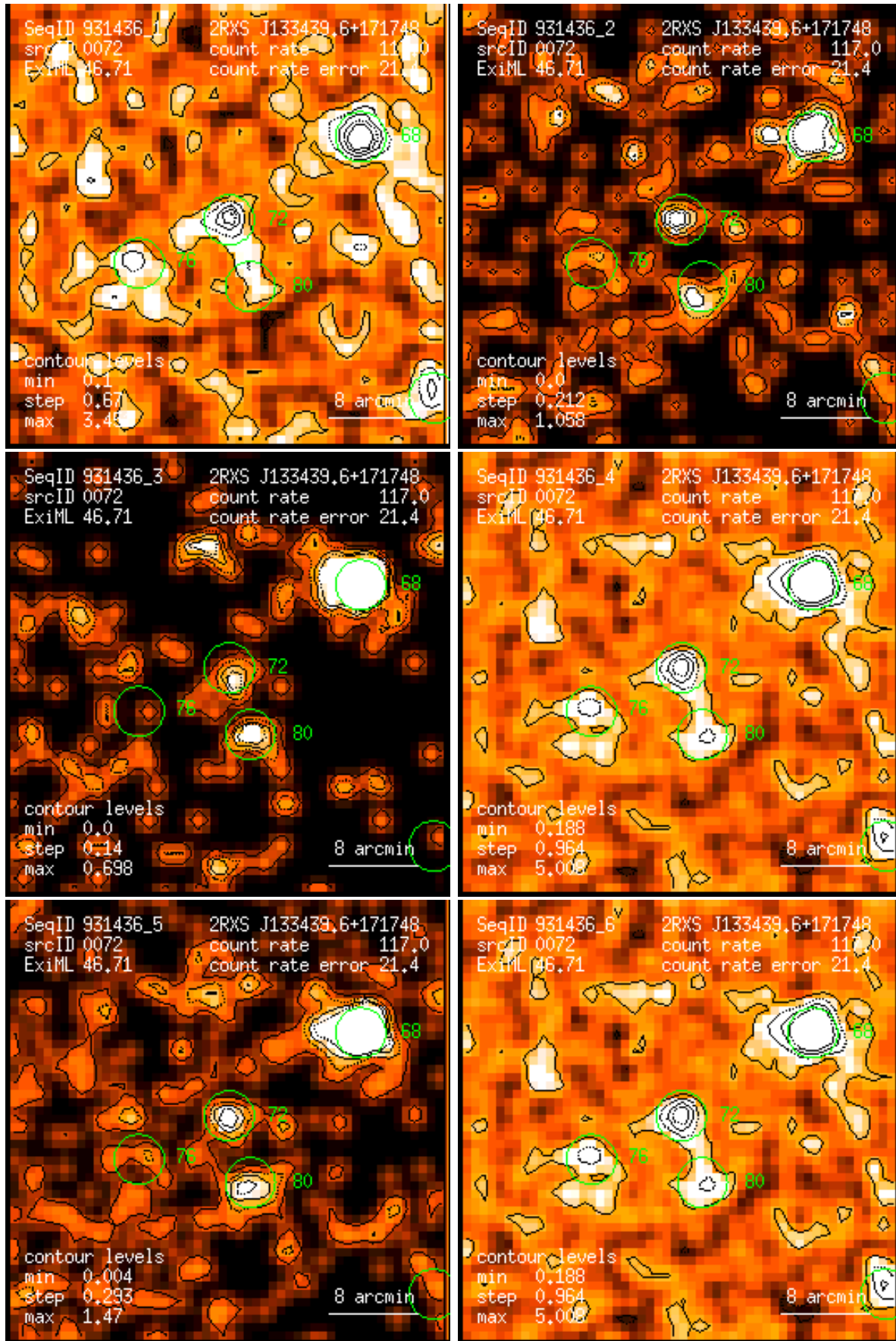
Figure 72: RASS 931436: detection 0072: band rate images, Gaussian filter: (1) PSPC channels 11 – 41, (2) 52 – 90, (3) 91 – 201, (4) 11 – 235, (5) 52 – 201, (6) 11 – 201. Broad band rates in counts/ks. Band rate contour levels in counts/ks/arcmin 2 .
