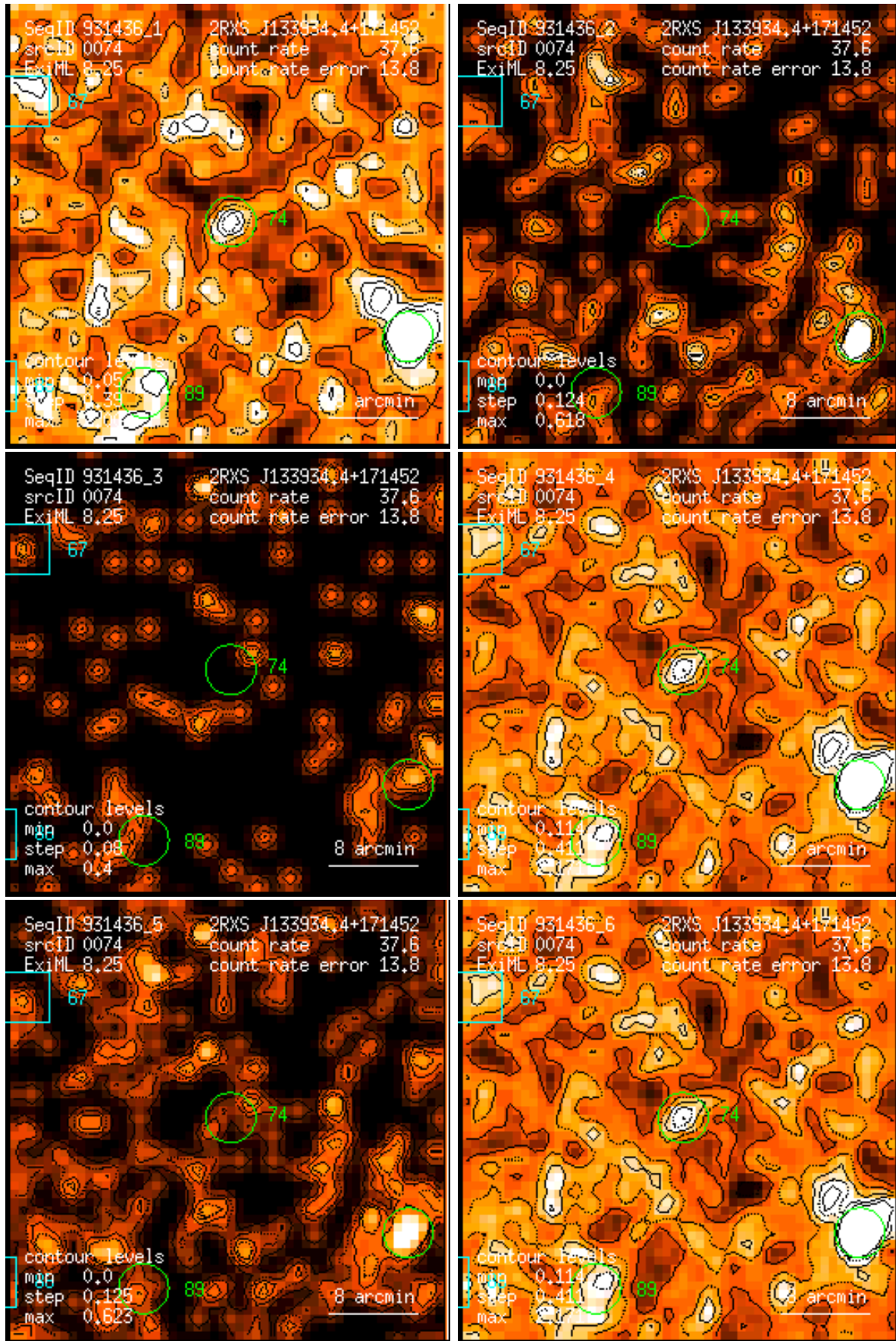
Figure 74: RASS 931436: detection 0074: band rate images, Gaussian filter: (1) PSPC channels 11 – 41, (2) 52 – 90, (3) 91 – 201, (4) 11 – 235, (5) 52 – 201, (6) 11 – 201. Broad band rates in counts/ks. Band rate contour levels in counts/ks/arcmin 2 .
