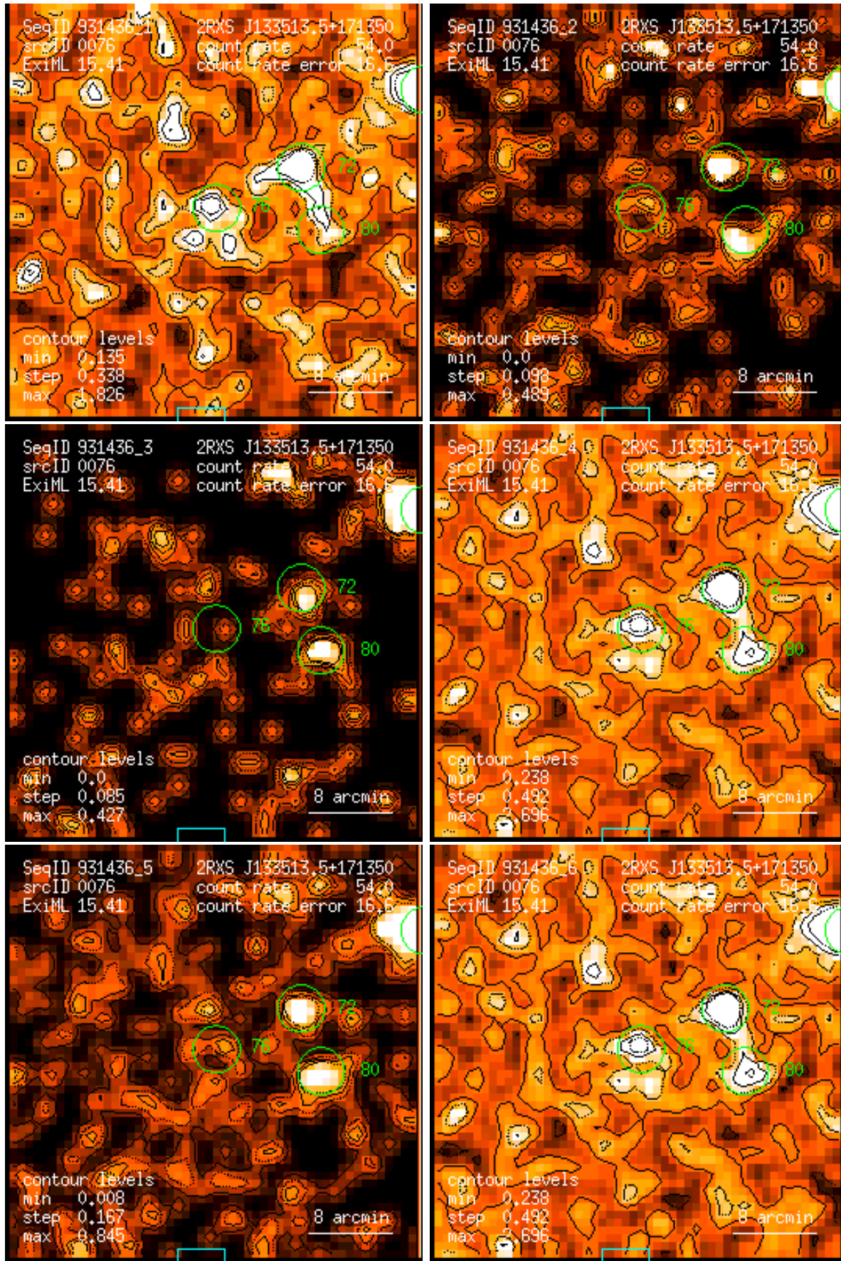
Figure 76: RASS 931436: detection 0076: band rate images, Gaussian filter: (1) PSPC channels 11 – 41, (2) 52 – 90, (3) 91 – 201, (4) 11 – 235, (5) 52 – 201, (6) 11 – 201. Broad band rates in counts/ks. Band rate contour levels in counts/ks/arcmin 2 .
