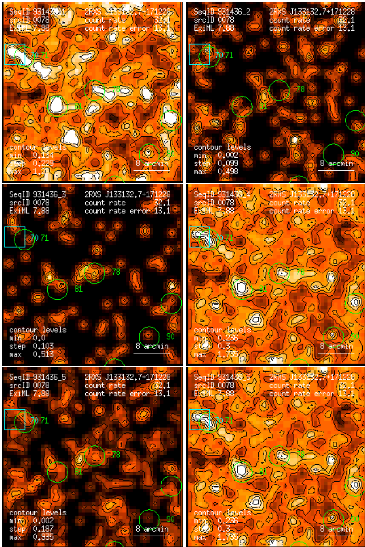
Figure 78: RASS 931436: detection 0078: band rate images, Gaussian filter: (1) PSPC channels 11 – 41, (2) 52 – 90, (3) 91 – 201, (4) 11 – 235, (5) 52 – 201, (6) 11 – 201. Broad band rates in counts/ks. Band rate contour levels in counts/ks/arcmin 2 .
