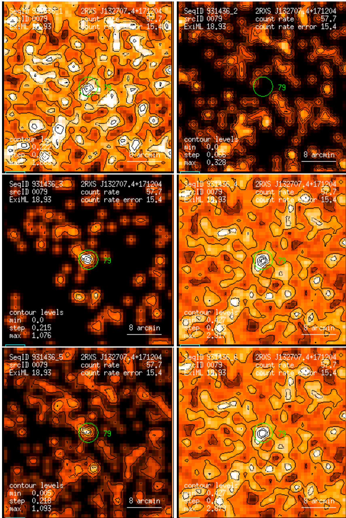
Figure 79: RASS 931436: detection 0079: band rate images, Gaussian filter: (1) PSPC channels 11 – 41, (2) 52 – 90, (3) 91 – 201, (4) 11 – 235, (5) 52 – 201, (6) 11 – 201. Broad band rates in counts/ks. Band rate contour levels in counts/ks/arcmin 2 .
