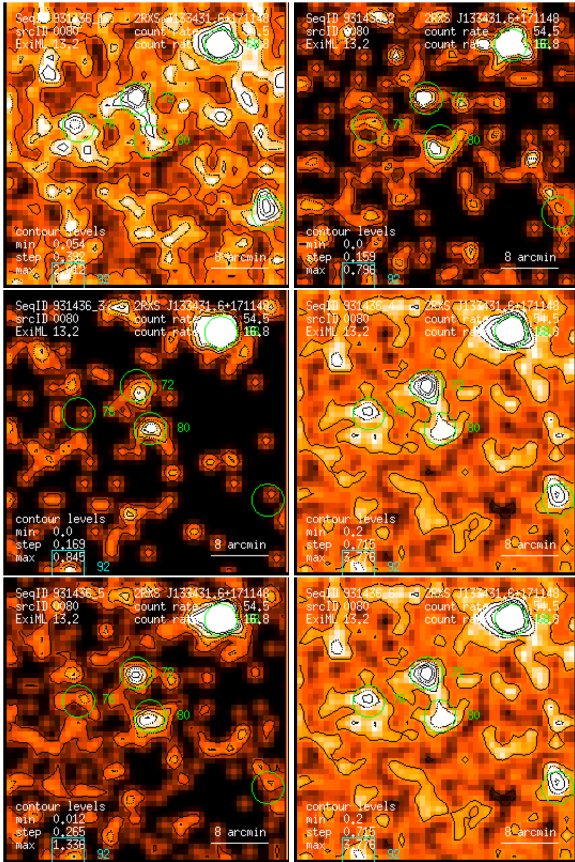
Figure 80: RASS 931436: detection 0080: band rate images, Gaussian filter: (1) PSPC channels 11 – 41, (2) 52 – 90, (3) 91 – 201, (4) 11 – 235, (5) 52 – 201, (6) 11 – 201. Broad band rates in counts/ks. Band rate contour levels in counts/ks/arcmin 2 .
