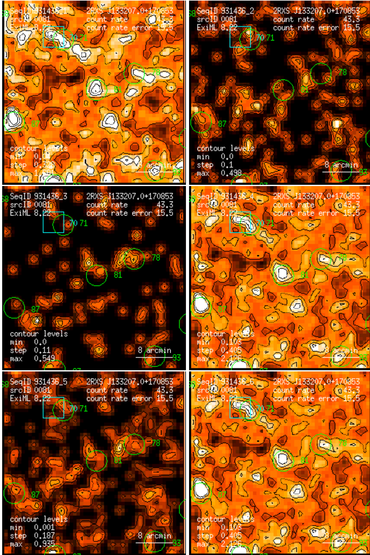
Figure 81: RASS 931436: detection 0081: band rate images, Gaussian filter: (1) PSPC channels 11 – 41, (2) 52 – 90, (3) 91 – 201, (4) 11 – 235, (5) 52 – 201, (6) 11 – 201. Broad band rates in counts/ks. Band rate contour levels in counts/ks/arcmin 2 .
